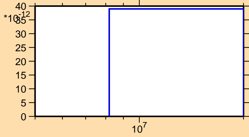
\sigma vs. E for ^{135}\text{Eu}(\text{mt 34})
