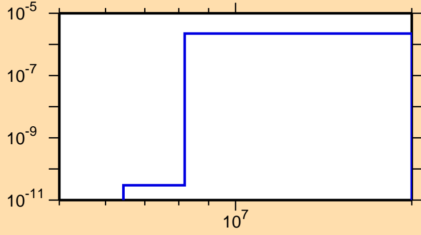
\sigma vs. E for ^{135}\text{Eu}(\text{mt117})
