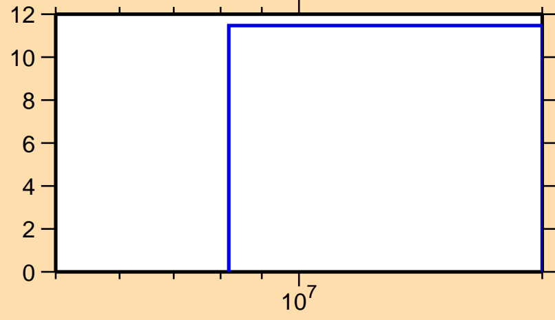
\Delta\sigma/\sigma vs. E for ^{135}\text{Eu}(n,\text{nonel.})
