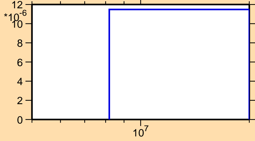
\sigma vs. E for ^{135}\text{Eu}(n,2np)
