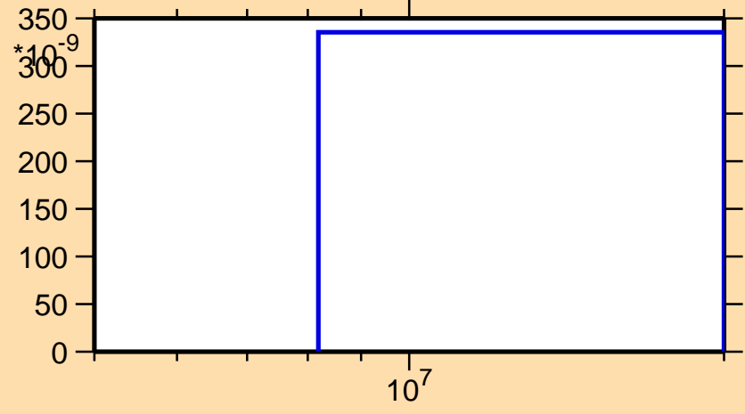
\sigma vs. E for ^{135}\text{Eu}(n,\text{pt})
