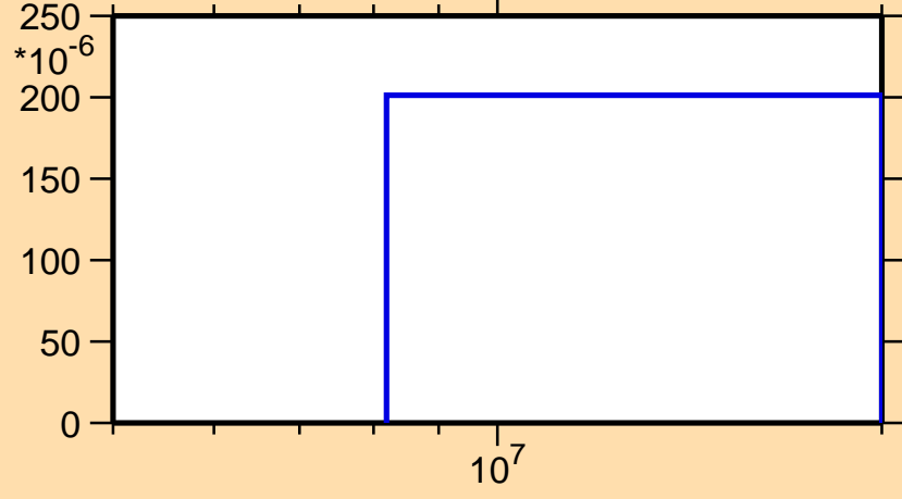
\sigma vs. E for ^{135}\text{Eu}(n,2n)
