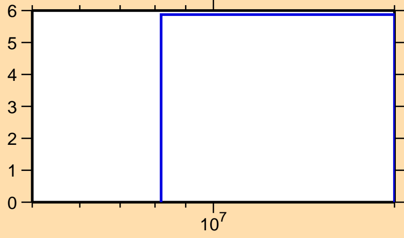
\Delta\sigma/\sigma vs. E for ^{135}\text{Eu}(n,\text{tot.})
