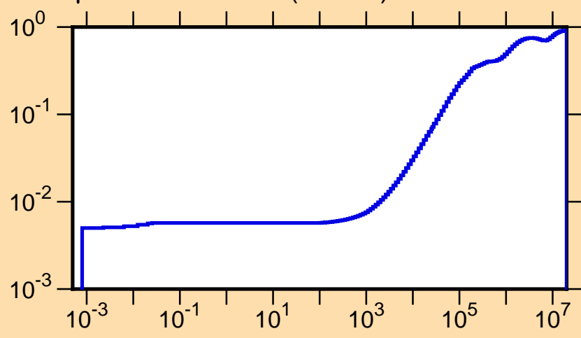
\mu vs. E for ^{136}\text{Eu}(\text{mt251})
