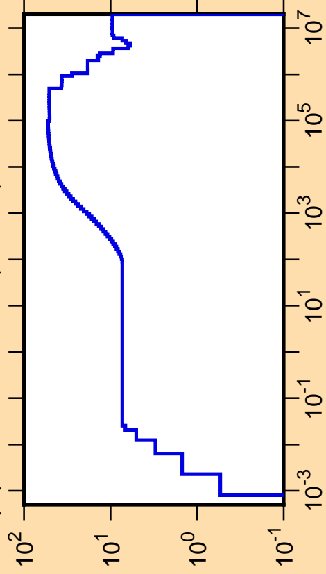
\Delta\mu/\mu vs. E for ^{136}\text{Eu}(\text{mt251})
