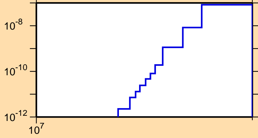
\sigma vs. E for ^{136}\text{Eu} (mt 34)
