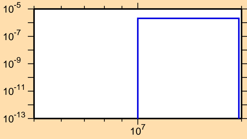
\sigma vs. E for ^{136}\text{Eu}(n,\text{nd})
