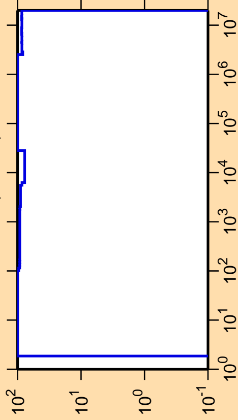
\Delta\sigma/\sigma vs. E for ^{136}\text{Eu}(n,\text{inel.})
