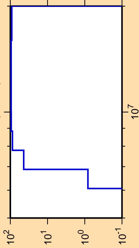
\Delta\sigma/\sigma vs. E for ^{136}\text{Eu} (mt 45)
