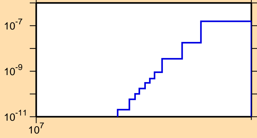
\sigma vs. E for ^{136}\text{Eu}(n,2n\alpha)
