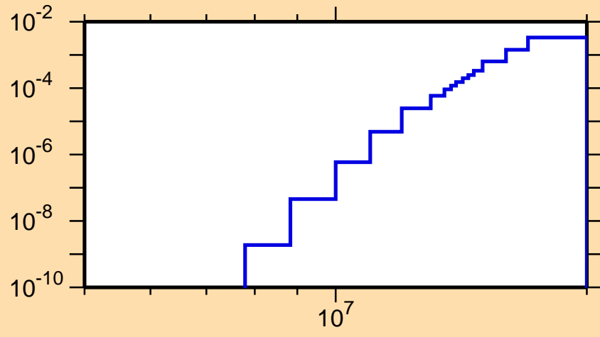
\sigma vs. E for ^{136}\text{Eu} (mt 45)
