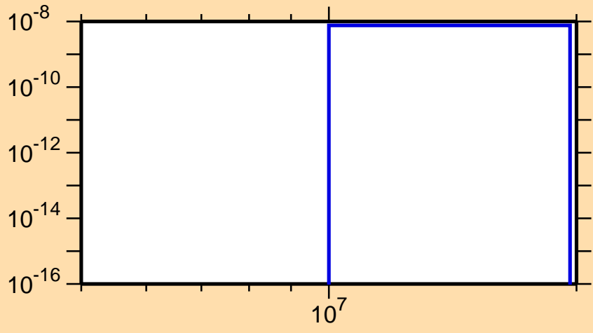
\sigma vs. E for ^{136}\text{Eu}(\text{mt } 34)
