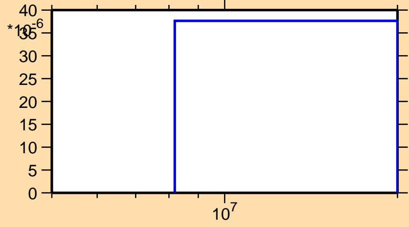
\sigma vs. E for ^{136}\text{Eu}(n,\text{pt})
