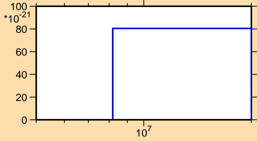
\sigma vs. E for ^{136}\text{Eu}(\text{mt 11})
