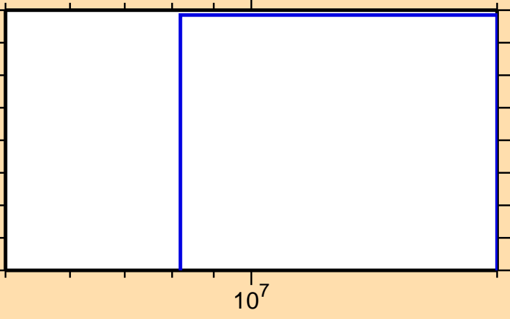
\sigma vs. E for ^{136}\text{Eu}(n,2n)
