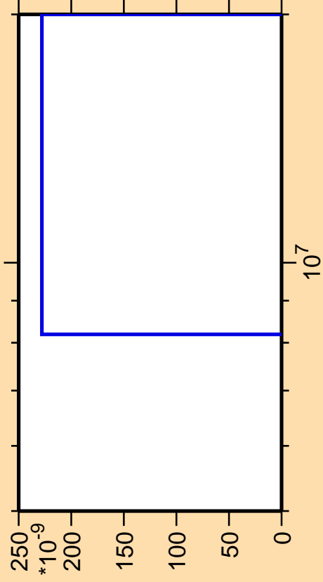
\Delta\sigma/\sigma vs. E for ^{136}\text{Eu}(\text{mt 11})
