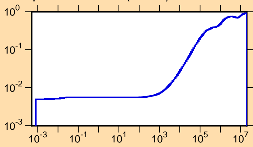
\mu vs. E for ^{137}\text{Eu}(\text{mt251})
