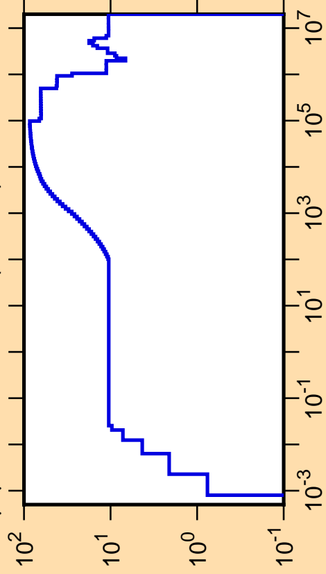
\Delta\mu/\mu vs. E for ^{137}\text{Eu}(\text{mt251})
