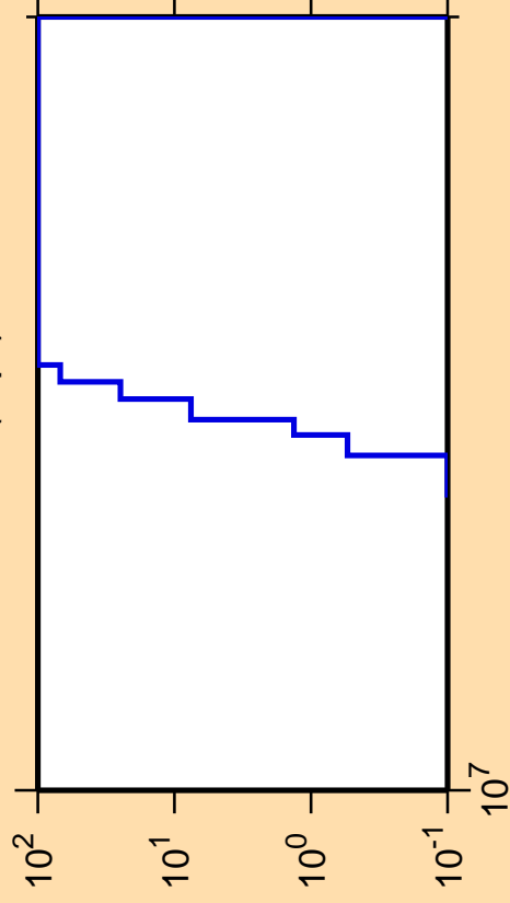
\Delta\sigma/\sigma vs. E for ^{137}\text{Eu}(n,\text{pt})
