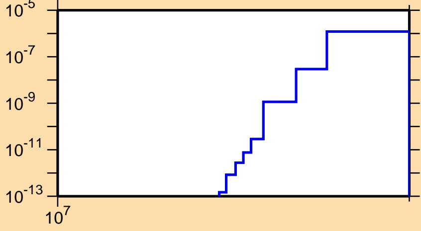
\sigma vs. E for ^{137}\text{Eu}(n,\text{pt})
