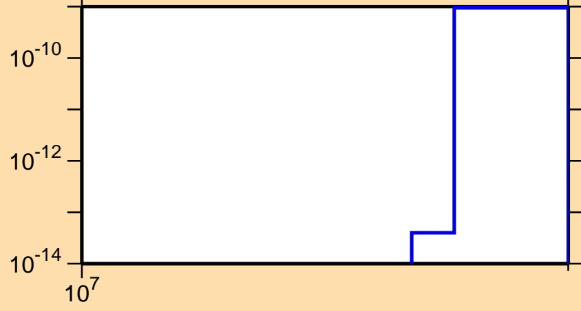
\sigma vs. E for ^{137}\text{Eu}(n,nt)
