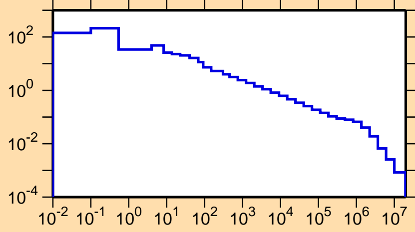
\sigma vs. E for ^{137}\text{Eu}(n,\gamma)
