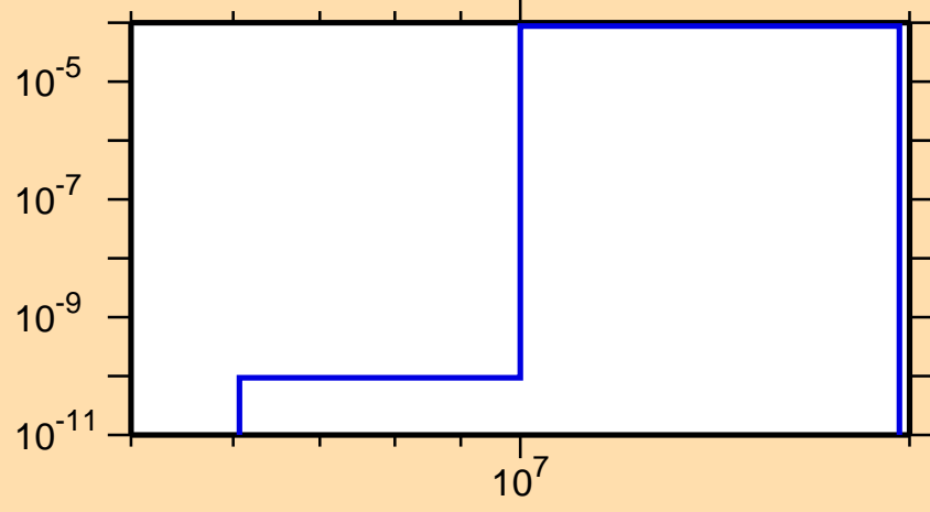
\sigma vs. E for ^{137}\text{Eu} (mt 45)
