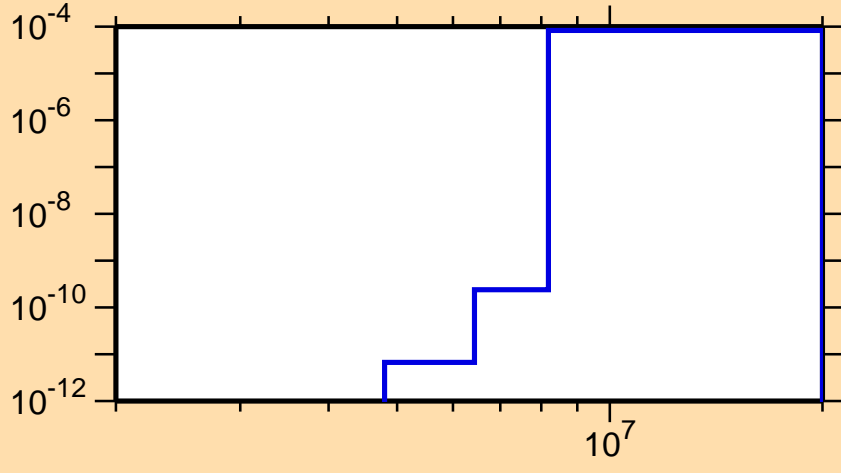
\sigma vs. E for ^{137}\text{Eu}(n,\text{He3})
