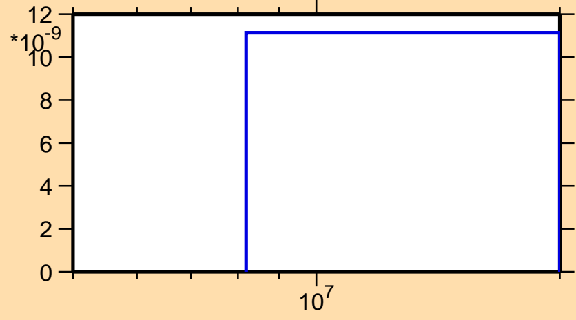
\sigma vs. E for ^{137}\text{Eu}(n,pt)
