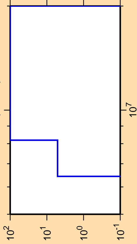
\Delta\sigma/\sigma vs. E for ^{137}\text{Eu} (mt 45)
