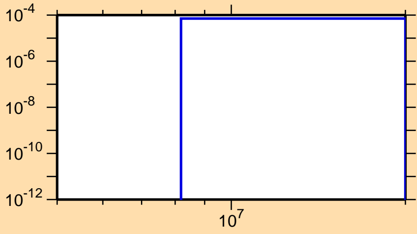
\sigma vs. E for ^{137}\text{Eu} (mt 45)
