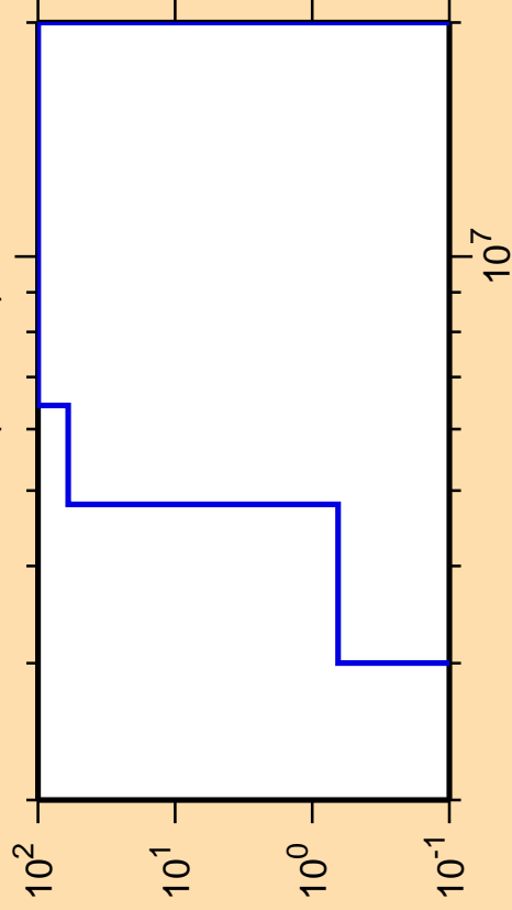
\Delta\sigma/\sigma vs. E for ^{137}\text{Eu}(n,\text{He3})
