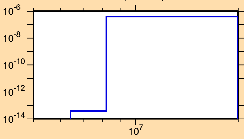
\sigma vs. E for ^{137}\text{Eu}(\text{mt117})
