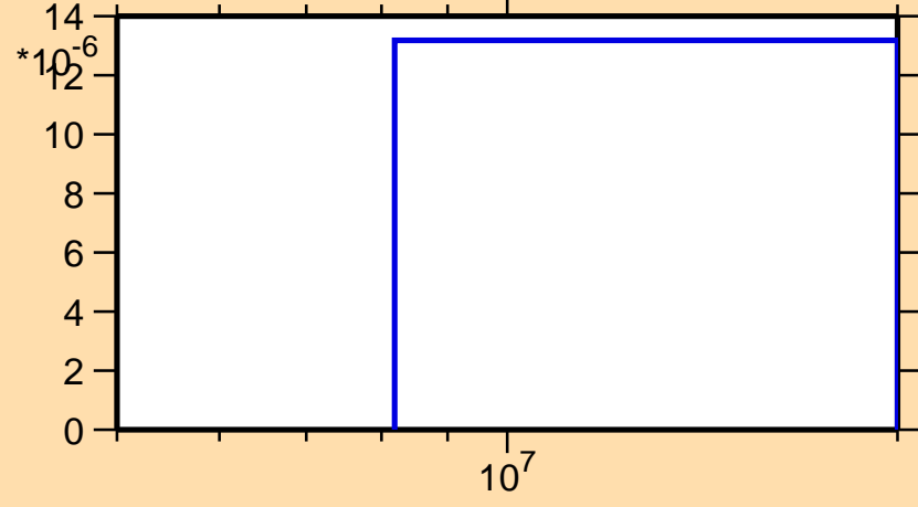
\sigma vs. E for ^{137}\text{Eu}(n,2np)
