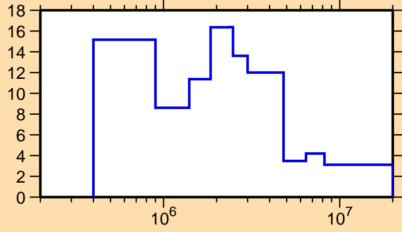
\Delta\sigma/\sigma vs. E for ^{137}\text{Eu}(n,tot.)
