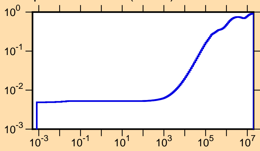
\mu vs. E for ^{139}\text{Eu}(\text{mt251})
