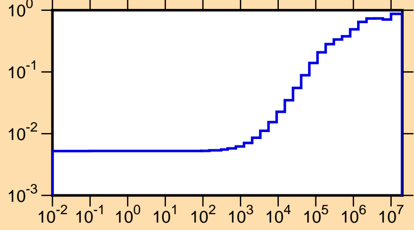
\mu vs. E for ^{139}\text{Eu}(\text{mt251})
