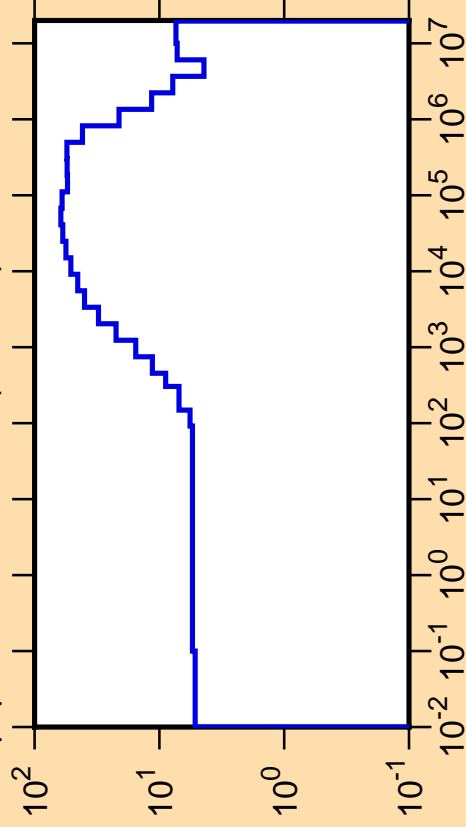
\Delta\mu/\mu vs. E for ^{139}\text{Eu}(\text{mt251})
