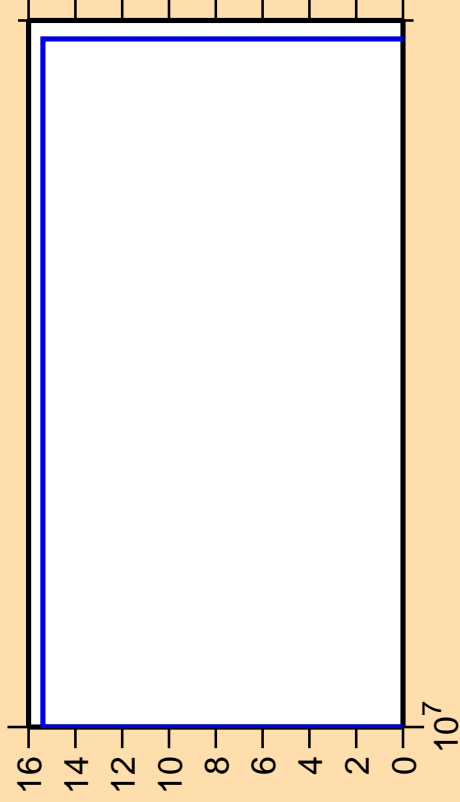
\Delta\sigma/\sigma vs. E for ^{139}\text{Eu} (mt 34)
