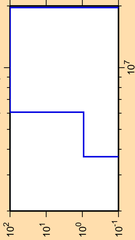
\Delta\sigma/\sigma vs. E for ^{139}\text{Eu}(n,\text{He3})
