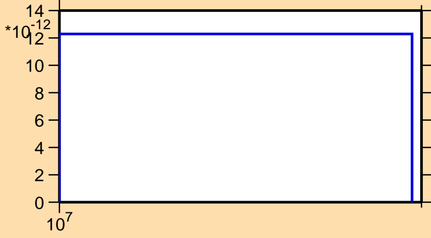
\sigma vs. E for ^{139}\text{Eu}(n,nt)
