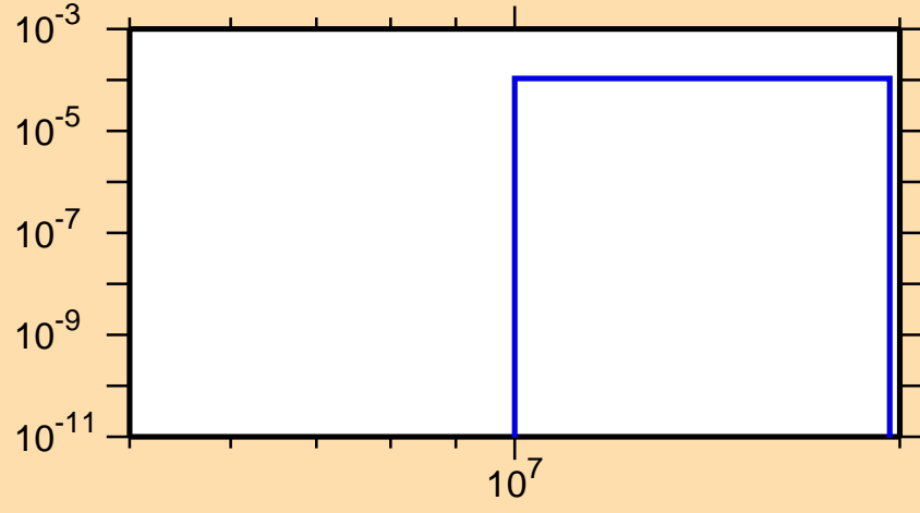
\sigma vs. E for ^{139}\text{Eu} (mt 45)
