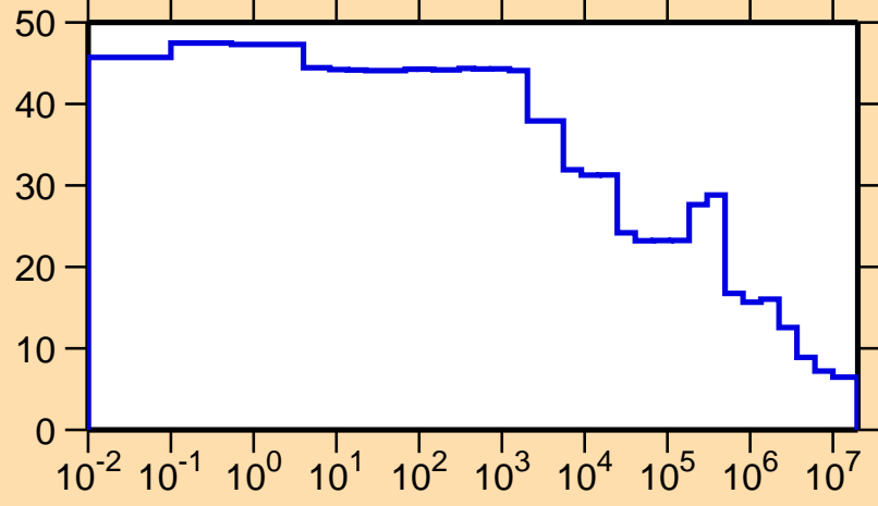
\Delta\sigma/\sigma vs. E for ^{139}\text{Eu}(n,\text{nonel.})
