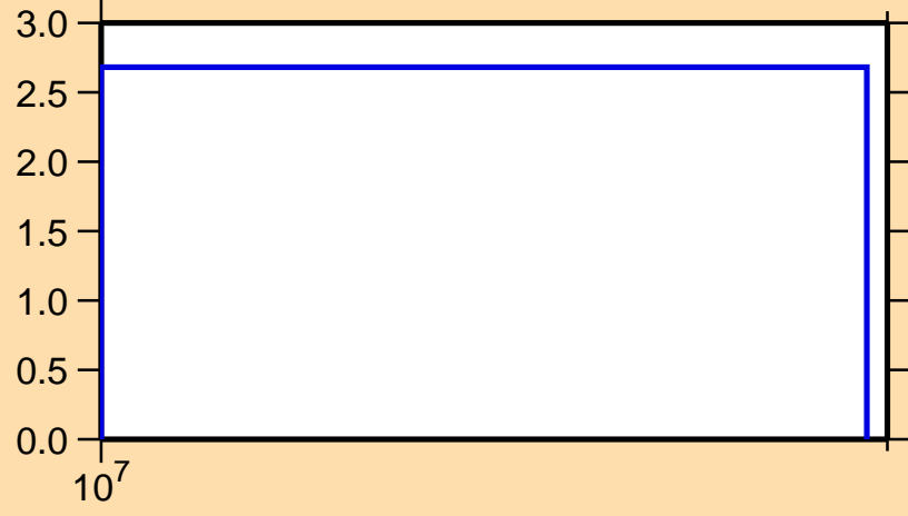
\Delta\sigma/\sigma vs. E for ^{139}\text{Eu}(n,\text{tot.})
