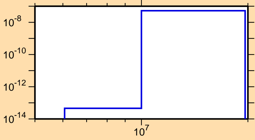
\sigma vs. E for ^{139}\text{Eu}(\text{mt117})
