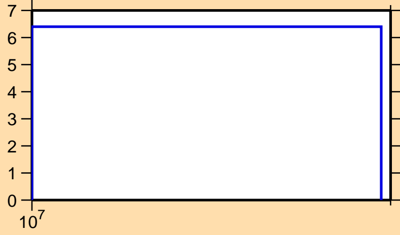
\Delta\sigma/\sigma vs. E for ^{139}\text{Eu}(n,\text{el.})
