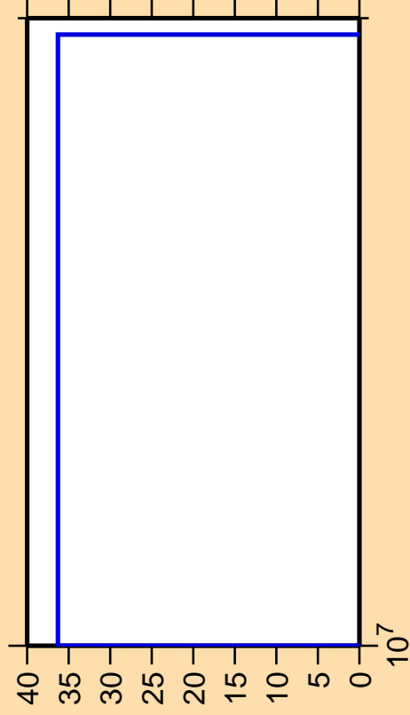
\Delta\sigma/\sigma vs. E for ^{139}\text{Eu}(n,p)
