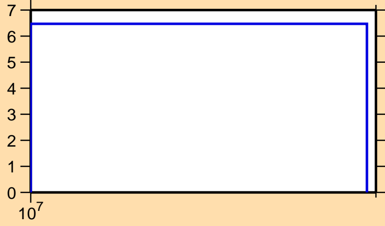
\Delta\sigma/\sigma vs. E for ^{139}\text{Eu}(n,\text{nonel.})
