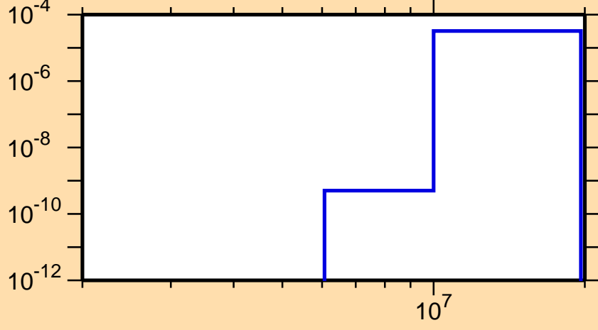
\sigma vs. E for ^{139}\text{Eu}(n,\text{He3})
