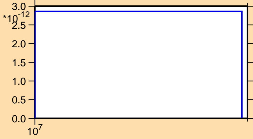
\sigma vs. E for ^{139}\text{Eu} (mt 34)
