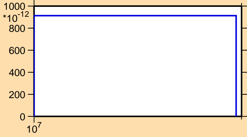
\sigma vs. E for ^{139}\text{Eu}(n,\text{pt})
