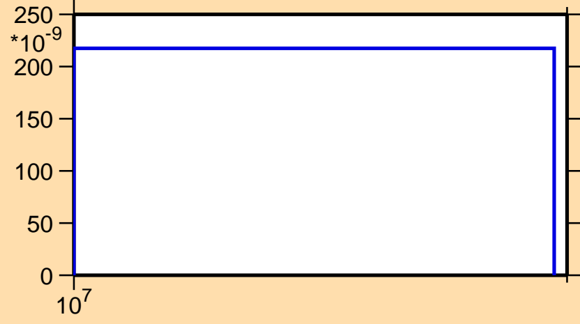
\sigma vs. E for ^{139}\text{Eu}(n,nd)
