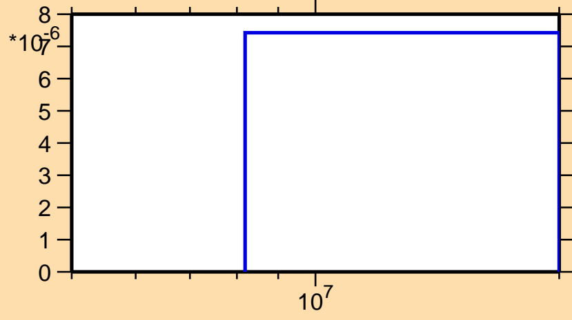
\sigma vs. E for ^{139}\text{Eu}(n,\text{pd})
