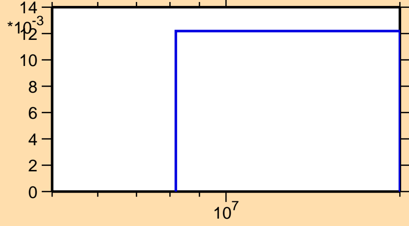
\sigma vs. E for ^{139}\text{Eu}(n,2n)
