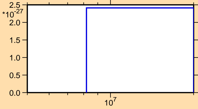
\sigma vs. E for ^{139}\text{Eu} (mt 11)
