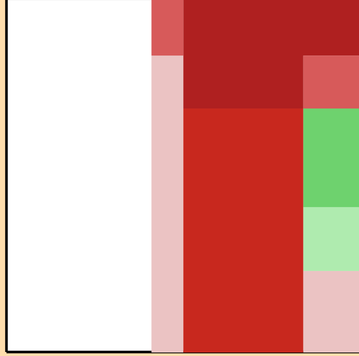
\Delta\sigma/\sigma vs. E for ^{140}\text{Eu}(n,2n)
