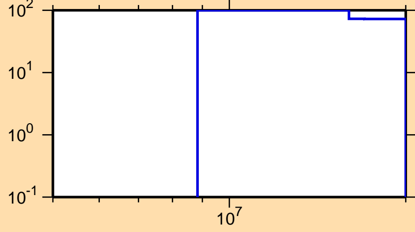
\Delta\sigma/\sigma vs. E for ^{140}\text{Eu}(n,2n)
