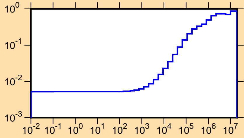
\mu vs. E for ^{140}\text{Eu}(\text{mt251})
