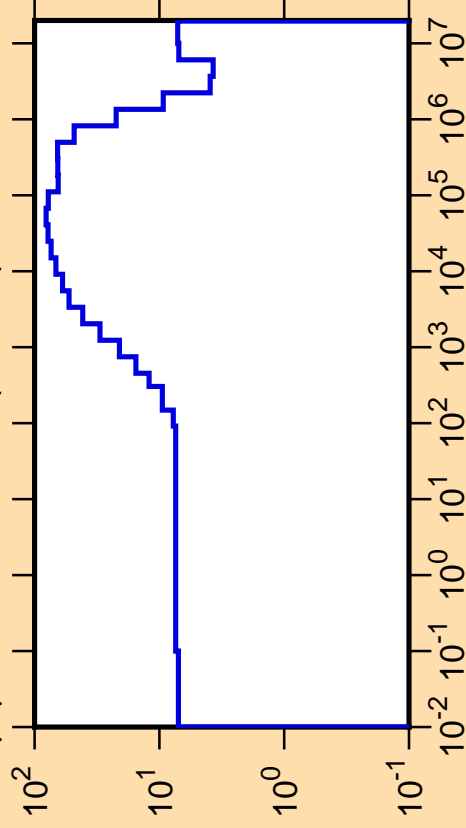
\Delta\mu/\mu vs. E for ^{140}\text{Eu}(\text{mt251})
