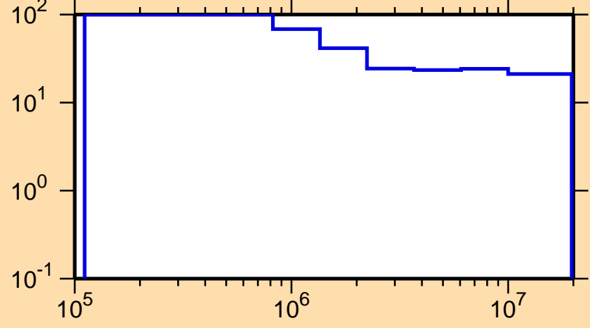
\Delta\sigma/\sigma vs. E for ^{140}\text{Eu}(n,\text{inel.})
