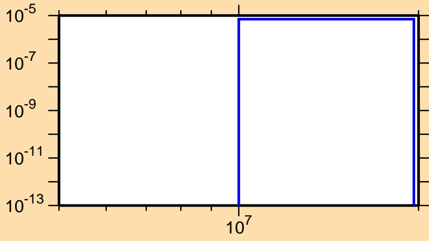
\sigma vs. E for ^{140}\text{Eu} (mt 45)
