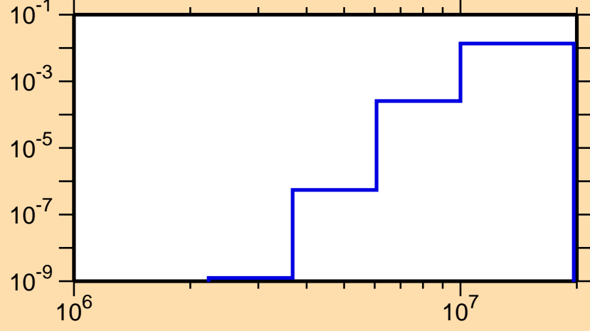
\sigma vs. E for ^{140}\text{Eu}(n,d)
