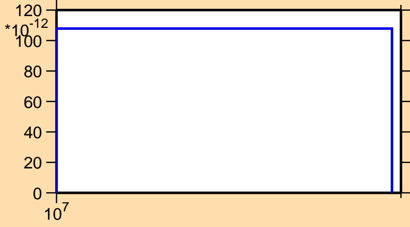
\sigma vs. E for ^{140}\text{Eu} (mt 34)
