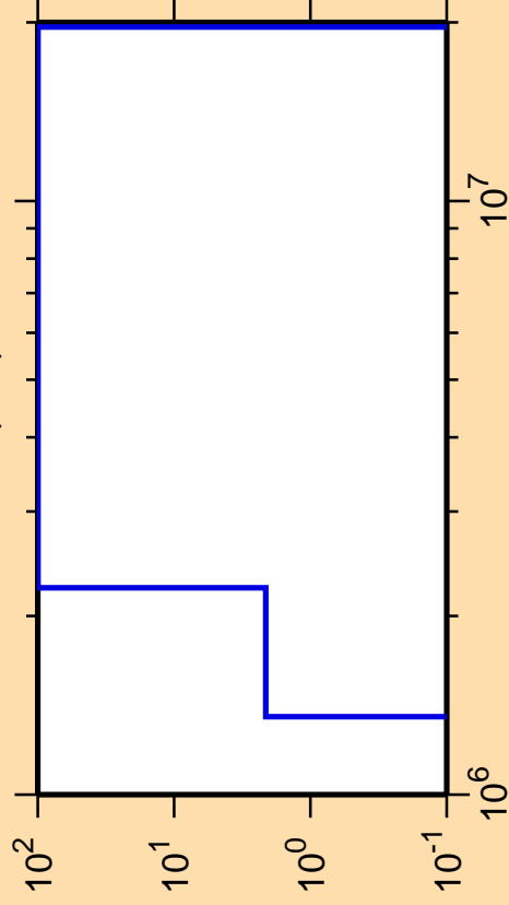
\Delta\sigma/\sigma vs. E for ^{140}\text{Eu}(n,d)
