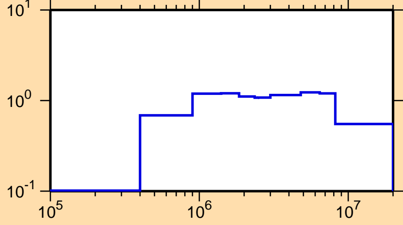
\sigma vs. E for ^{140}\text{Eu}(n,\text{inel.})
