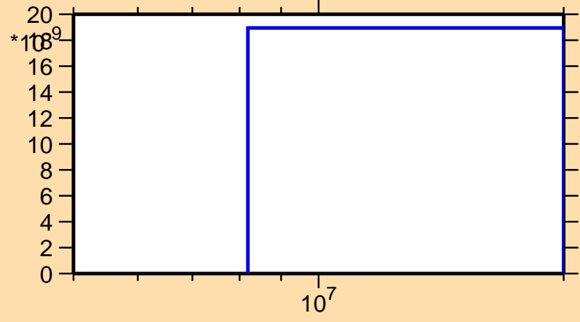
\sigma vs. E for ^{140}\text{Eu}(n,\text{pt})
