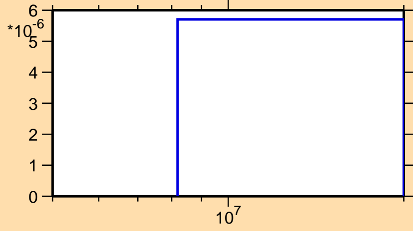
\sigma vs. E for ^{140}\text{Eu}(\text{mt } 45)
