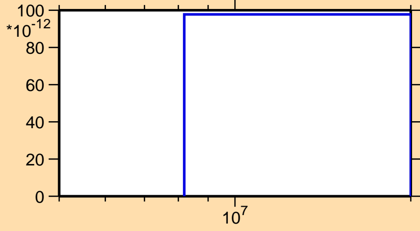
\sigma vs. E for ^{140}\text{Eu}(\text{mt } 34)
