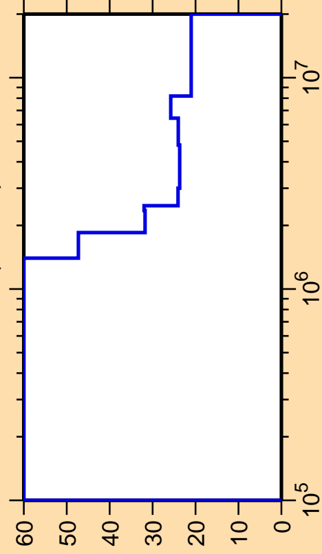
\Delta\sigma/\sigma vs. E for ^{140}\text{Eu}(n,\text{inel.})
