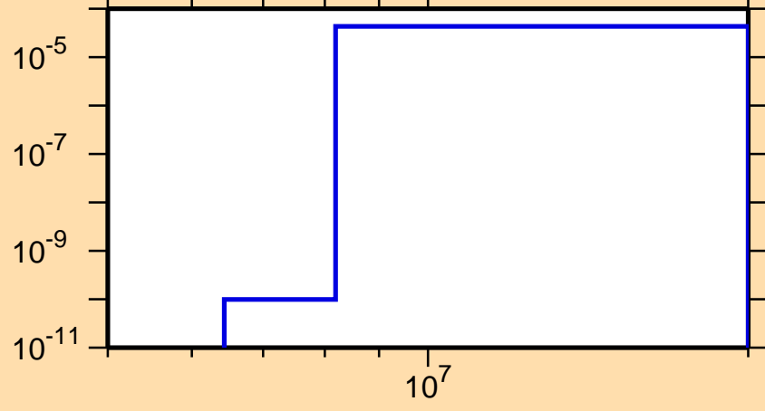
\sigma vs. E for ^{140}\text{Eu}(n,\text{He3})
