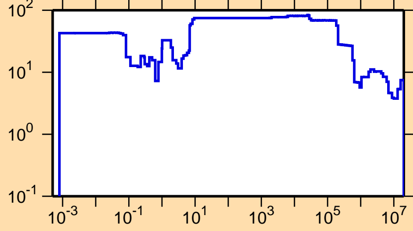
\Delta\sigma/\sigma vs. E for ^{141}\text{Eu}(n,\text{tot.})
