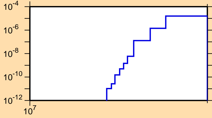
\sigma vs. E for ^{141}\text{Eu}(n,\text{nd})
