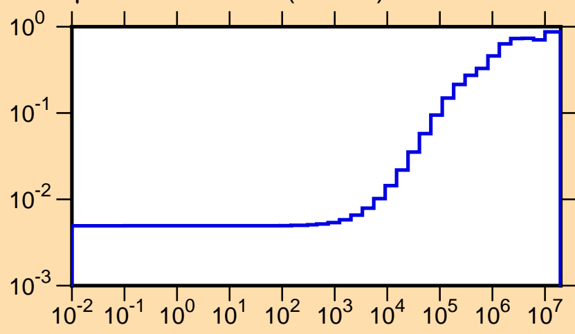
\mu vs. E for ^{141}\text{Eu}(\text{mt251})
