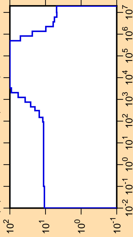
\Delta\mu/\mu vs. E for ^{141}\text{Eu}(\text{mt251})
