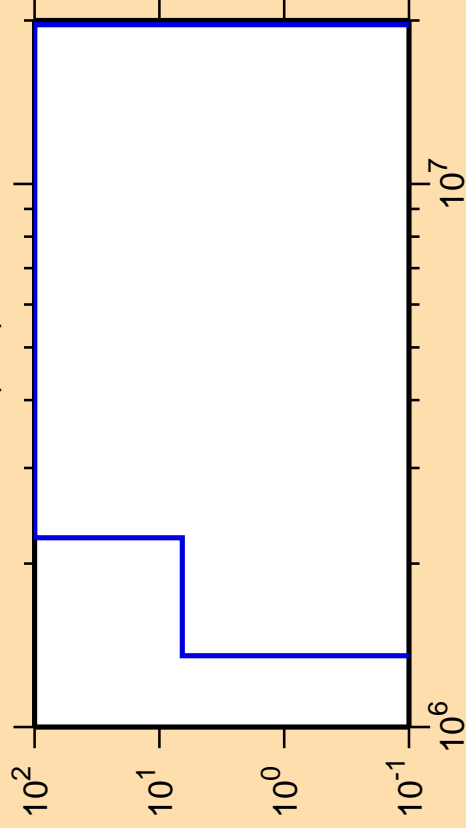
\Delta\sigma/\sigma vs. E for ^{141}\text{Eu}(n,d)
