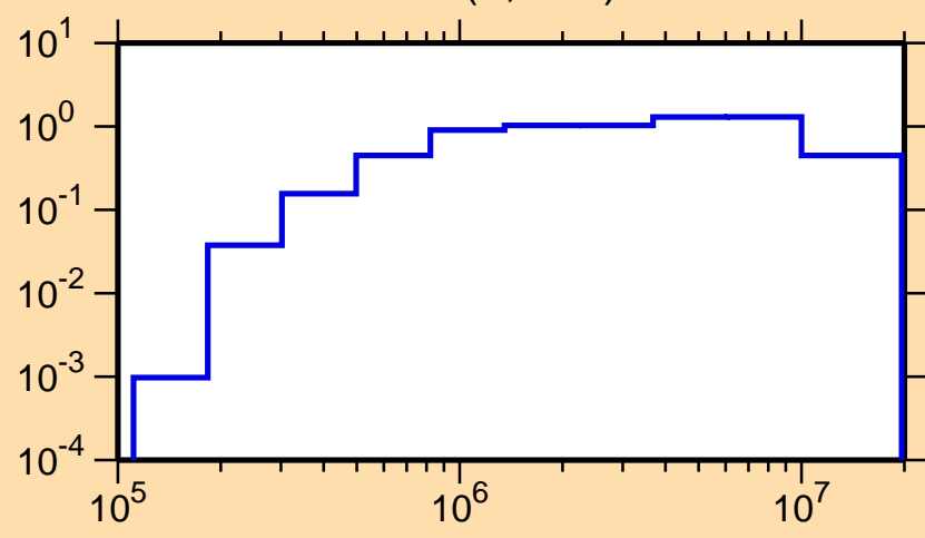
\sigma vs. E for ^{141}\text{Eu}(n,\text{inel.})
