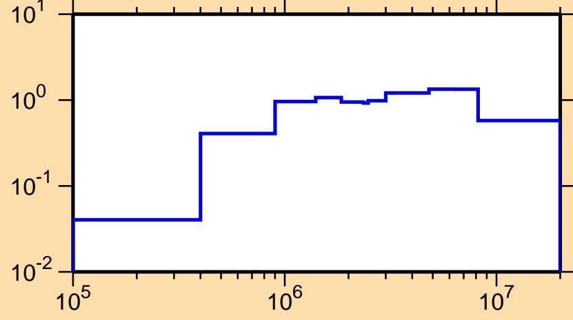
\sigma vs. E for ^{141}\text{Eu}(n,\text{inel.})
