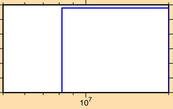
\sigma vs. E for ^{141}\text{Eu} (mt 34)
