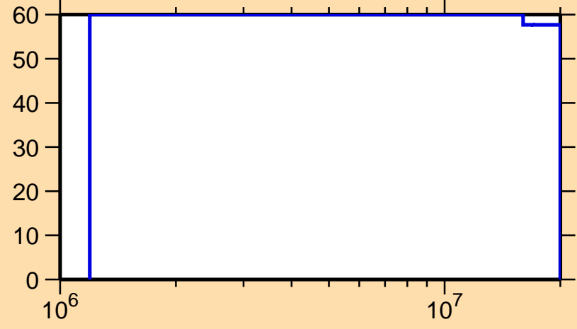
\Delta\sigma/\sigma vs. E for ^{141}\text{Eu}(n,ncont.)
