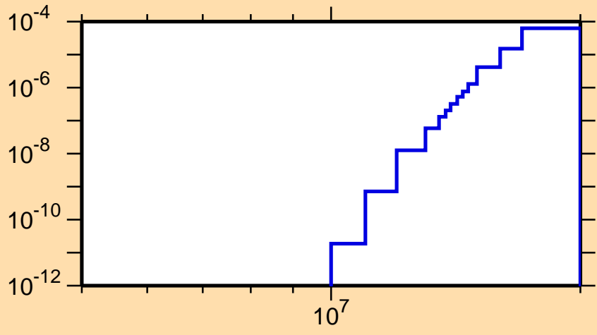
\sigma vs. E for ^{141}\text{Eu} (mt 45)
