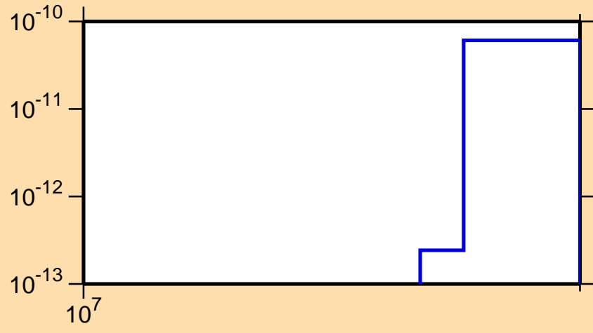
\sigma vs. E for ^{141}\text{Eu} (mt 34)
