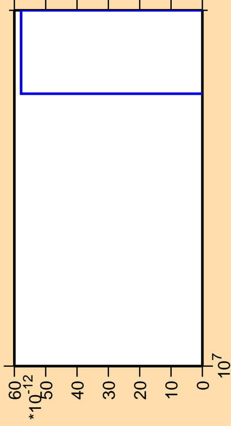
\Delta\sigma/\sigma vs. E for ^{141}\text{Eu} (mt 11)
