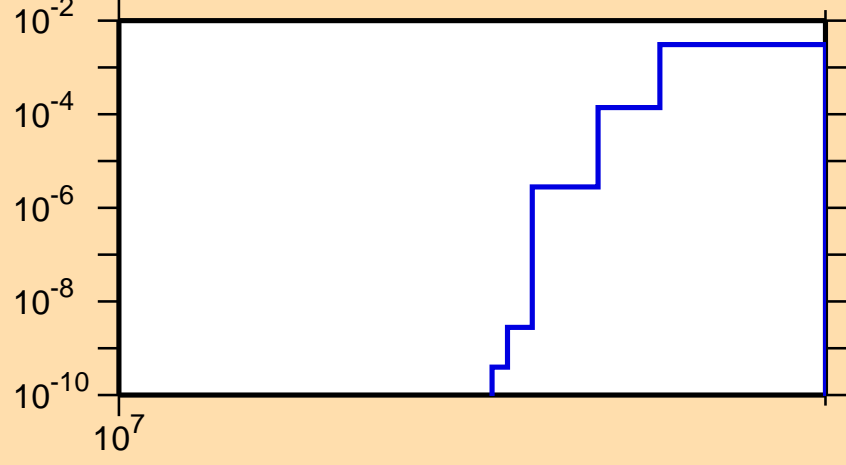
\sigma vs. E for ^{141}\text{Eu}(n,2np)
