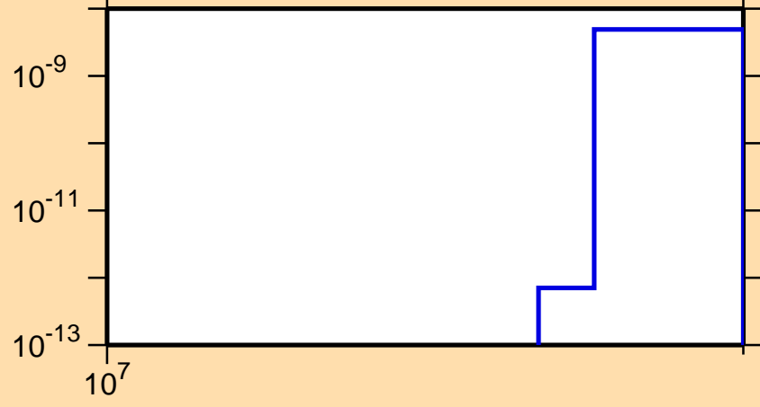
\sigma vs. E for ^{141}\text{Eu}(n,nt)
