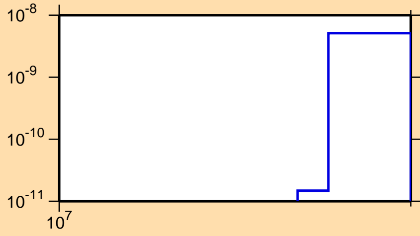
\sigma vs. E for ^{141}\text{Eu}(n,\text{pt})
