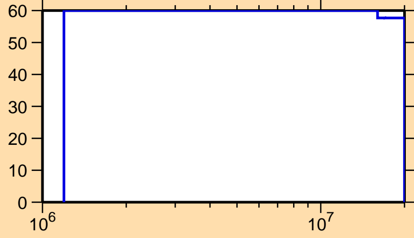
\Delta\sigma/\sigma vs. E for ^{141}\text{Eu}(n,n\text{cont.})
