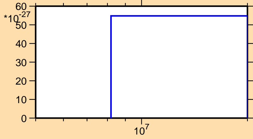
\sigma vs. E for ^{141}\text{Eu} (mt 11)
