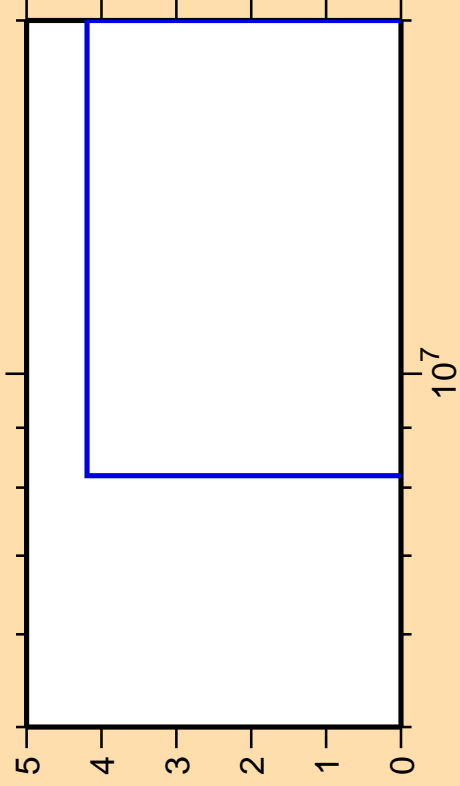
\Delta\sigma/\sigma vs. E for ^{141}\text{Eu} (mt 34)
