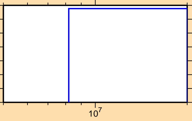
\sigma vs. E for ^{141}\text{Eu}(n,\text{nd})
