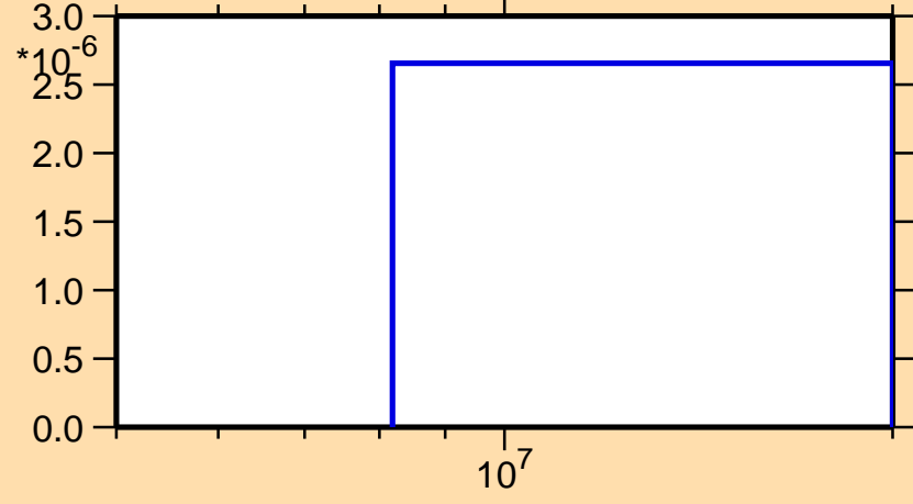
\sigma vs. E for ^{142}\text{Eu}(n,\text{nd})
