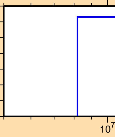
\sigma vs. E for ^{142}\text{Eu} (mt 34)
