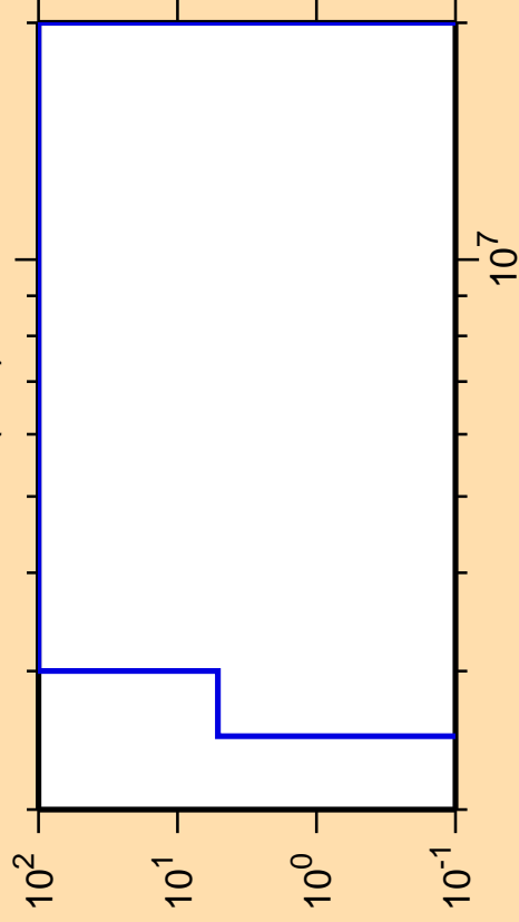
\Delta\sigma/\sigma vs. E for ^{142}\text{Eu}(n,d)
