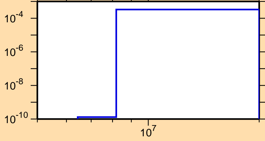
\sigma vs. E for ^{142}\text{Eu}(n,t)
