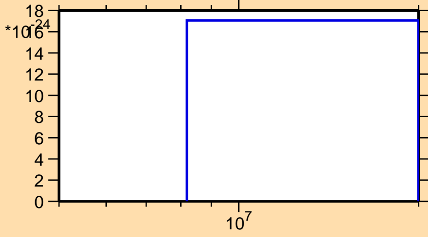
\sigma vs. E for ^{142}\text{Eu} (mt 11)
