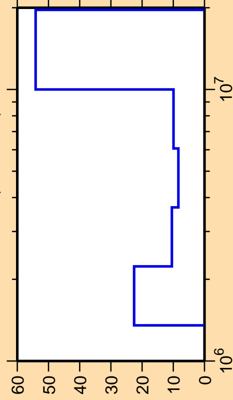
\Delta\sigma/\sigma vs. E for ^{143}\text{Eu}(n,\text{ncont.})
