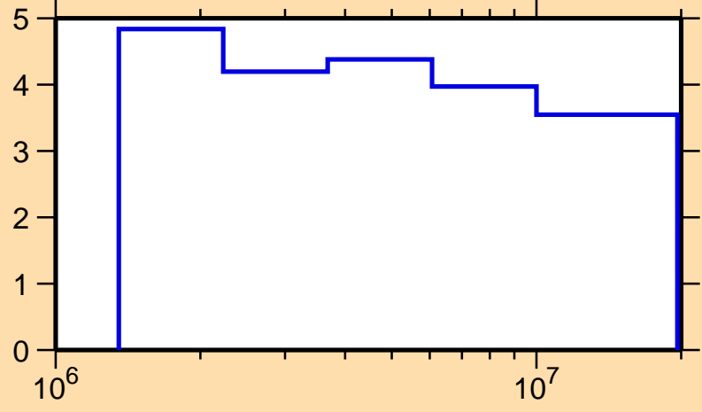
\Delta\sigma/\sigma vs. E for ^{143}\text{Eu}(n,n\text{nonel.})
