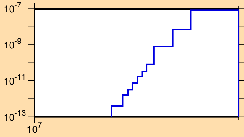
\sigma vs. E for ^{144}\text{Eu} (mt 45)
