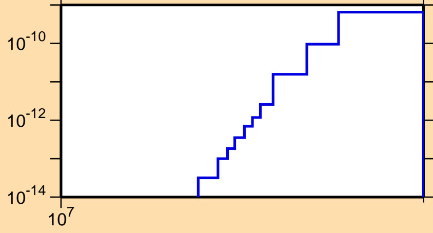
\sigma vs. E for ^{144}\text{Eu}(\text{mt117})
