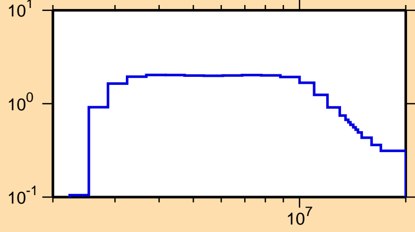
\sigma vs. E for ^{144}\text{Eu}(n,n\text{cont.})
