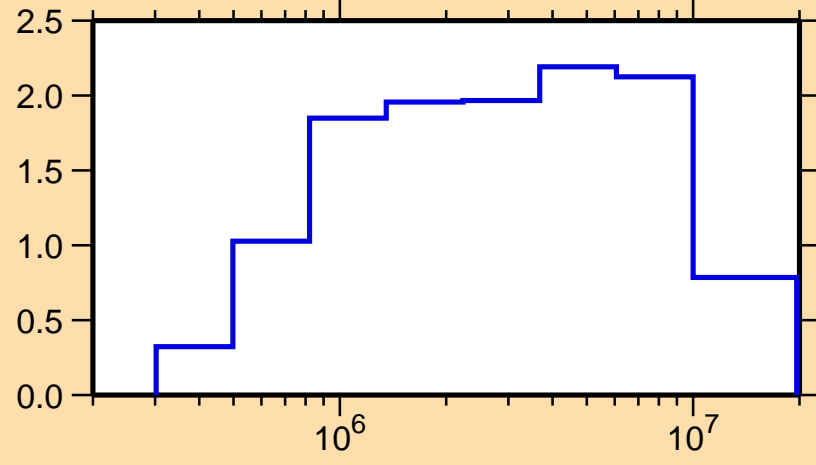
\sigma vs. E for ^{144}\text{Eu}(n,\text{inel.})
