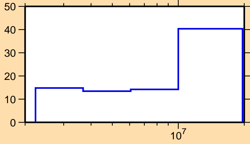
\Delta\sigma/\sigma vs. E for ^{144}\text{Eu}(n,ncont.)
