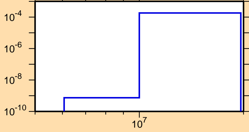
\sigma vs. E for ^{144}\text{Eu}(n,t)
