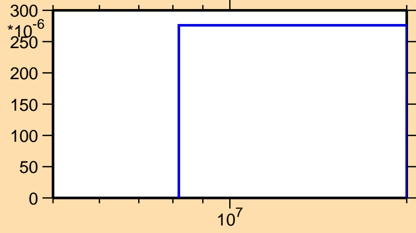
\sigma vs. E for ^{144}\text{Eu}(n,2np)
