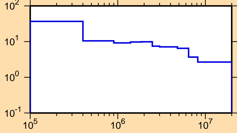
\Delta\sigma/\sigma vs. E for ^{144}\text{Eu}(n,\text{tot.})
