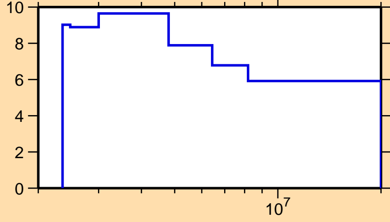
\Delta\sigma/\sigma vs. E for ^{144}\text{Eu}(n,n\text{nonel.})
