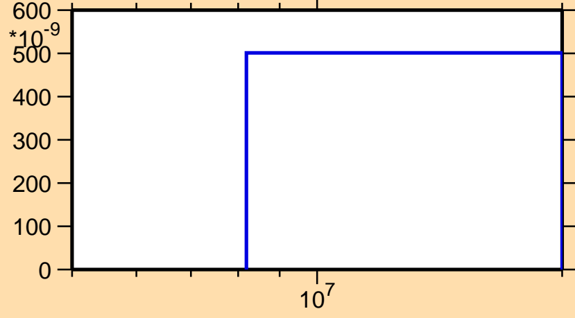
\sigma vs. E for ^{144}\text{Eu}(n,\text{nd})
