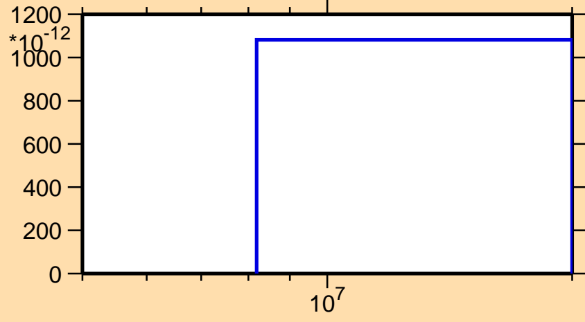
\sigma vs. E for ^{144}\text{Eu} (mt 45)
