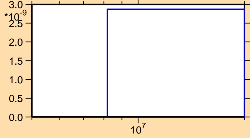
\sigma vs. E for ^{144}\text{Eu}(n,2n\alpha)
