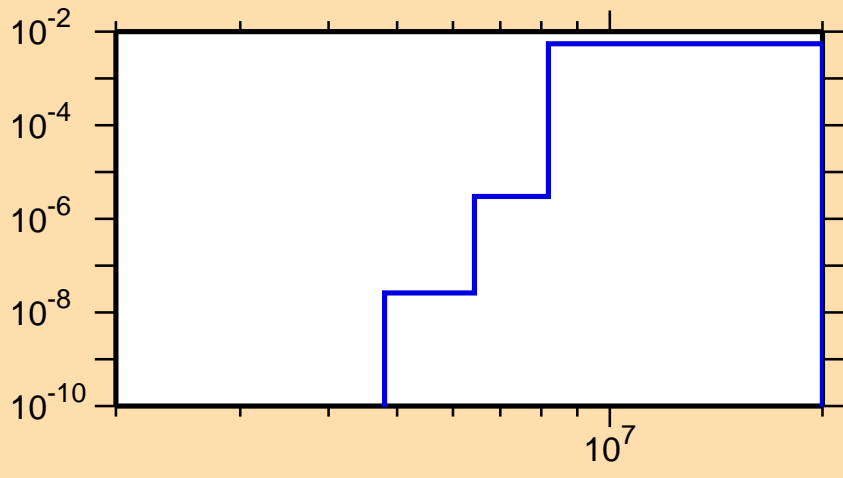
\sigma vs. E for ^{144}\text{Eu}(n,d)
