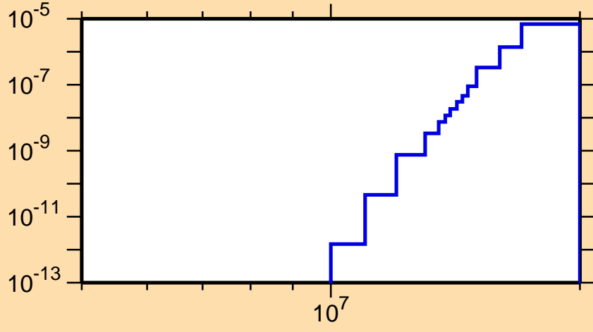
\sigma vs. E for ^{145}\text{Eu}(n,\text{He3})
