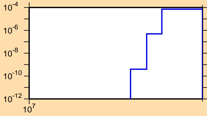
\sigma vs. E for ^{145}\text{Eu}(n,2np)
