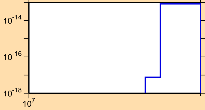
\sigma vs. E for ^{145}\text{Eu} (mt 34)
