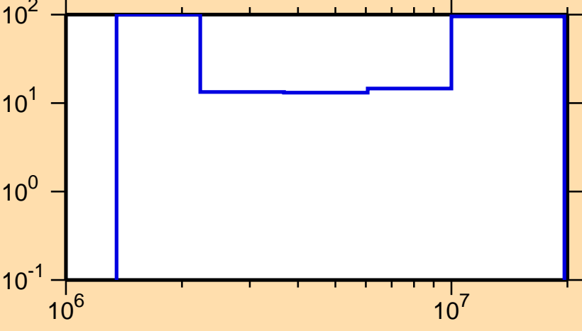
\Delta\sigma/\sigma vs. E for ^{145}\text{Eu}(n,n\text{cont.})
