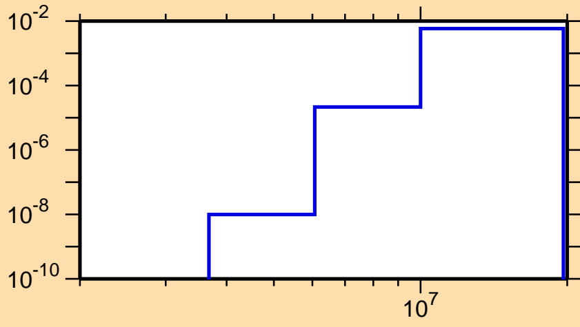
\sigma vs. E for ^{145}\text{Eu}(n,d)
