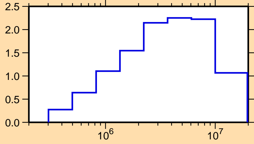
\sigma vs. E for ^{145}\text{Eu}(n,\text{inel.})
