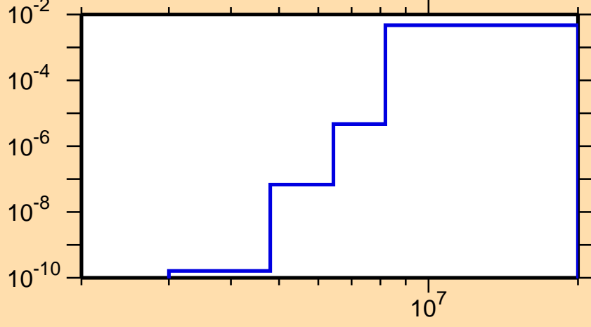
\sigma vs. E for ^{145}\text{Eu}(n,d)
