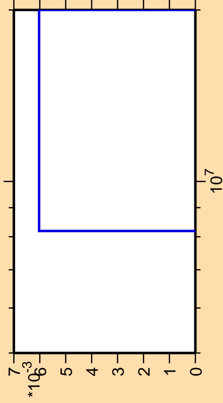
\Delta\sigma/\sigma vs. E for ^{145}\text{Eu} (mt 34)
