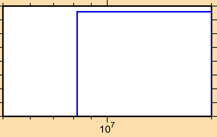
\sigma vs. E for ^{145}\text{Eu}(n,\text{pd})
