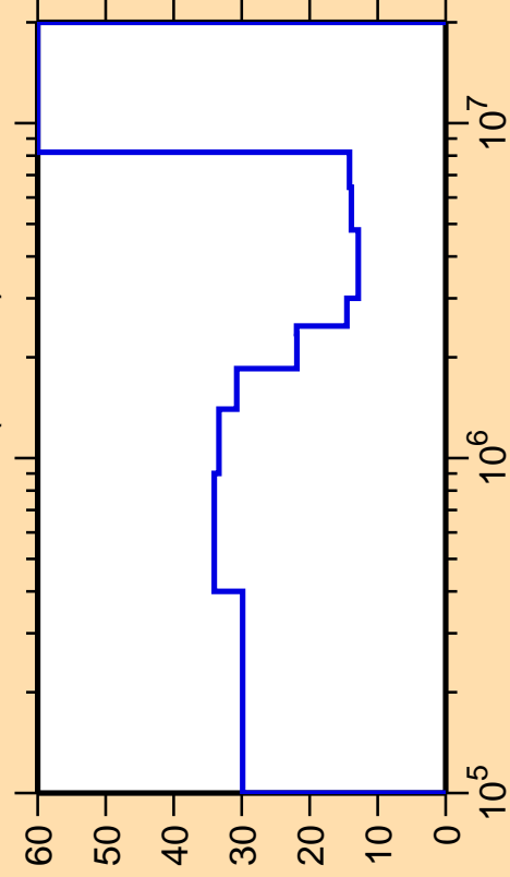
\Delta\sigma/\sigma vs. E for ^{145}\text{Eu}(n,\text{inel.})
