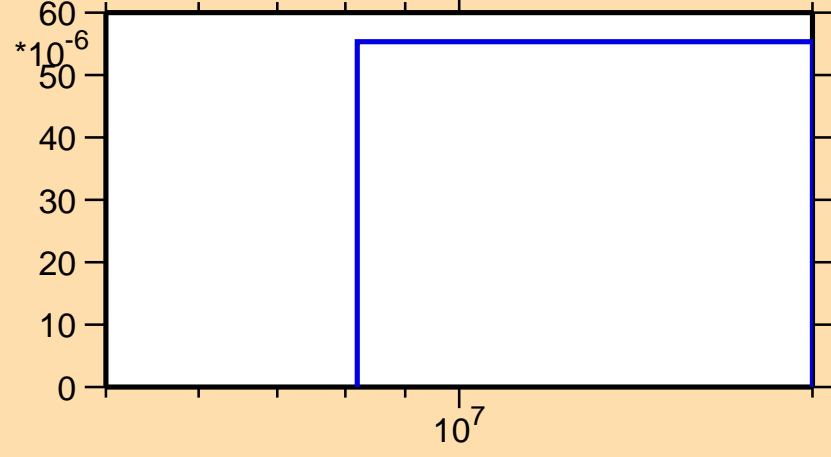
\sigma vs. E for ^{145}\text{Eu}(n,t)
