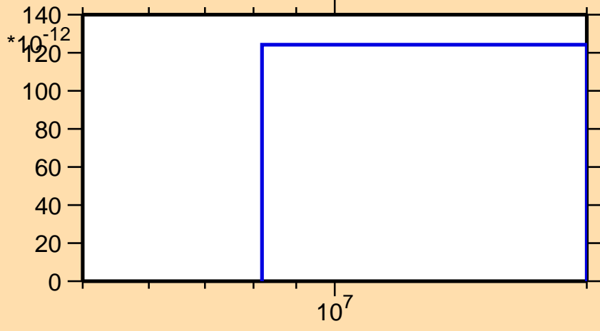
\sigma vs. E for ^{145}\text{Eu}(\text{mt } 45)
