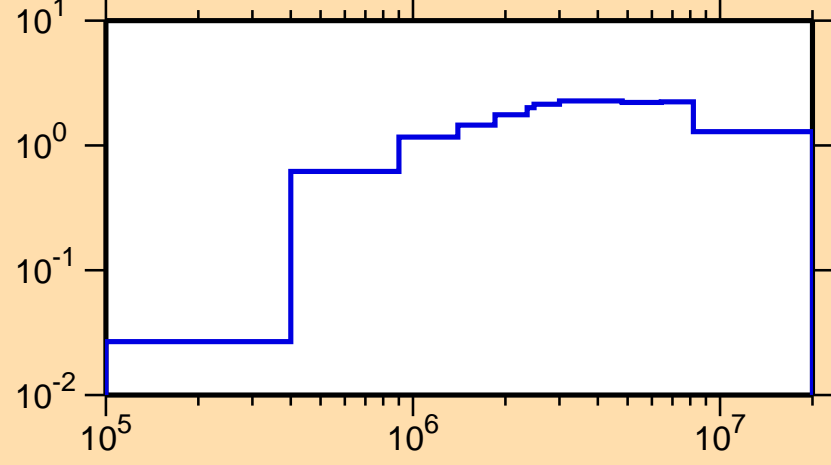
\sigma vs. E for ^{145}\text{Eu}(n,\text{inel.})
