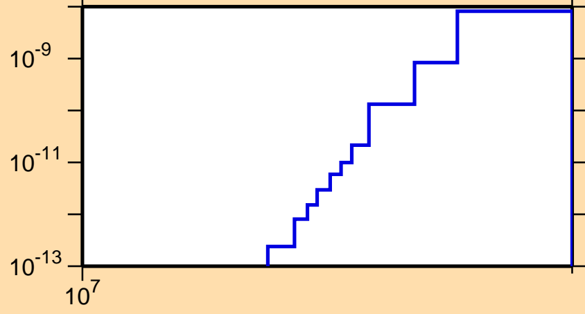
\sigma vs. E for ^{146}\text{Eu} (mt 45)
