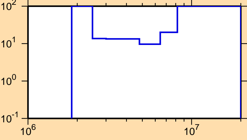
\Delta\sigma/\sigma vs. E for ^{146}\text{Eu}(n,n\text{cont.})
