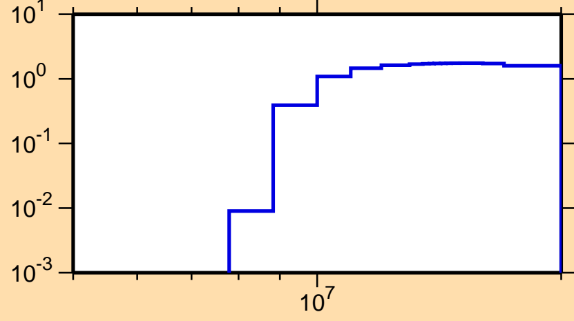
\sigma vs. E for ^{147}\text{Eu}(n,2n)
