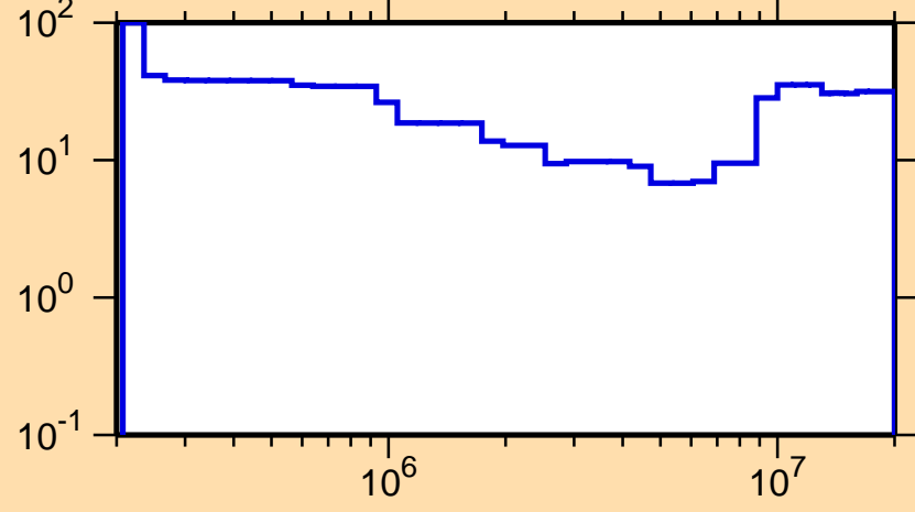
\Delta\sigma/\sigma vs. E for ^{147}\text{Eu}(n,\text{inel.})
