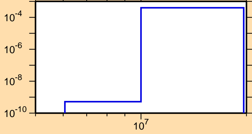
\sigma vs. E for ^{147}\text{Eu}(n,t)
