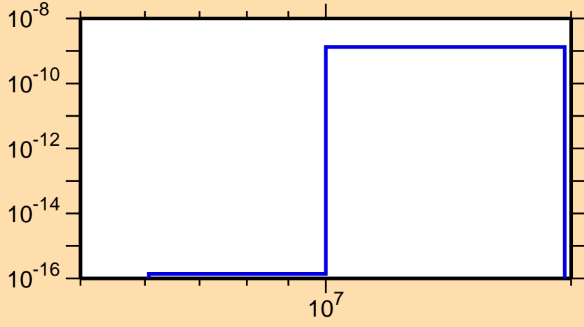
\sigma vs. E for ^{147}\text{Eu}(\text{mt117})
