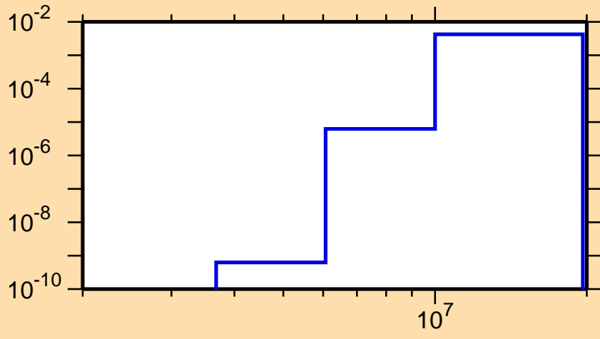
\sigma vs. E for ^{147}\text{Eu}(n,d)
