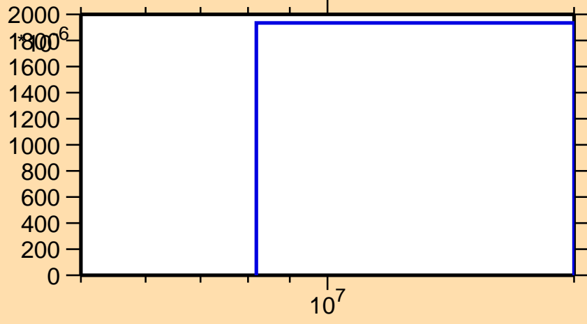
\sigma vs. E for ^{147}\text{Eu}(n,3n)
