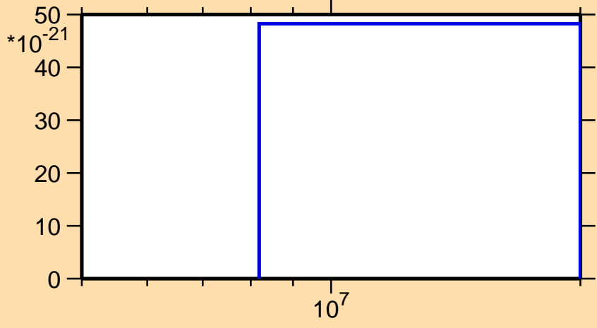
\sigma vs. E for ^{147}\text{Eu} (mt 42)
