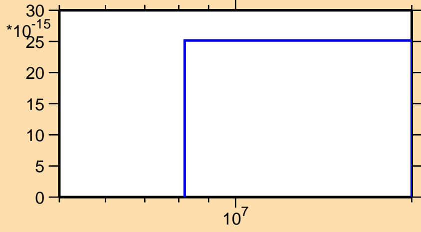
\sigma vs. E for ^{147}\text{Eu} (mt 34)
