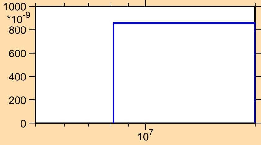
\sigma vs. E for ^{147}\text{Eu}(n,nd)
