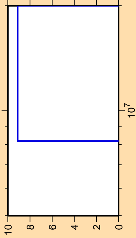
\Delta\sigma/\sigma vs. E for ^{147}\text{Eu}(n,2n)
