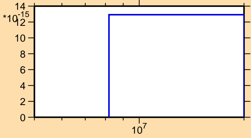
\sigma vs. E for ^{147}\text{Eu}(n,\text{pt})
