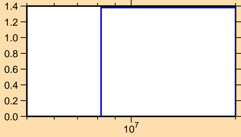
\sigma vs. E for ^{147}\text{Eu}(n,2n)
