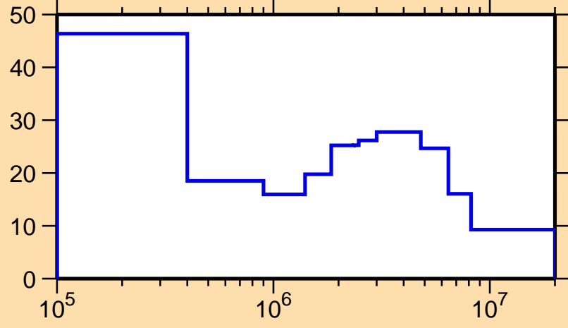
\Delta\sigma/\sigma vs. E for ^{147}\text{Eu}(n,\text{el.})
