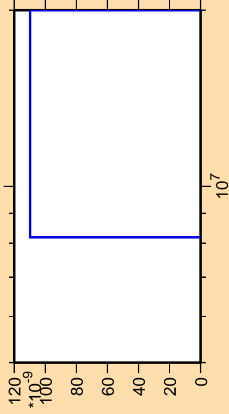
\Delta\sigma/\sigma vs. E for ^{147}\text{Eu} (mt 42)
