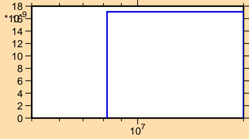
\sigma vs. E for ^{147}\text{Eu}(n,\text{He3})
