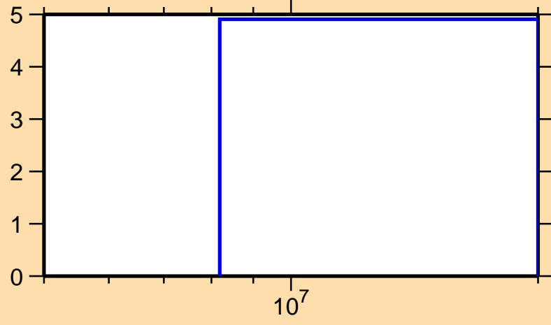
\Delta\sigma/\sigma vs. E for ^{147}\text{Eu}(n,\text{tot.})
