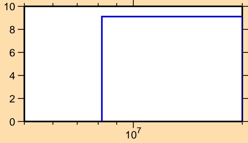
\Delta\sigma/\sigma vs. E for ^{147}\text{Eu}(n,2n)
