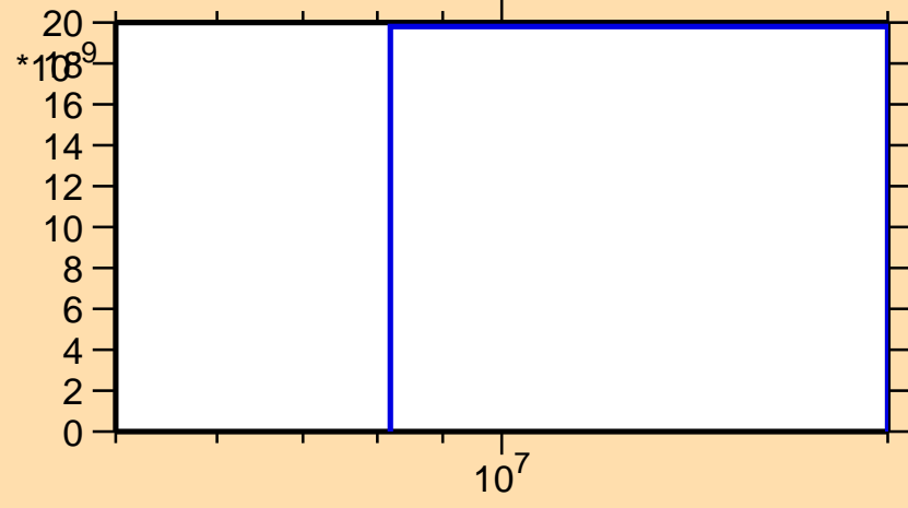
\sigma vs. E for ^{147}\text{Eu}(n,2n\alpha)
