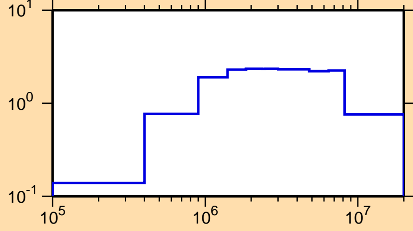
\sigma vs. E for ^{147}\text{Eu}(n,\text{inel.})
