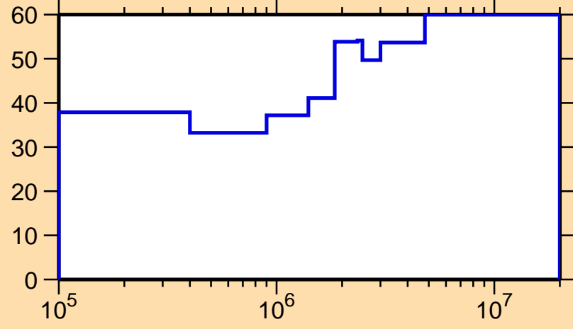
\Delta\sigma/\sigma vs. E for ^{147}\text{Eu}(n,n_1)
