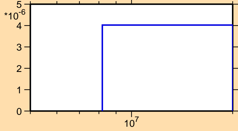
\sigma vs. E for ^{147}\text{Eu}(n,2np)
