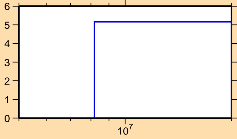
\Delta\sigma/\sigma vs. E for ^{147}\text{Eu}(n,\text{nonel.})
