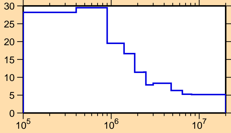
\Delta\sigma/\sigma vs. E for ^{147}\text{Eu}(n,\text{nonel.})
