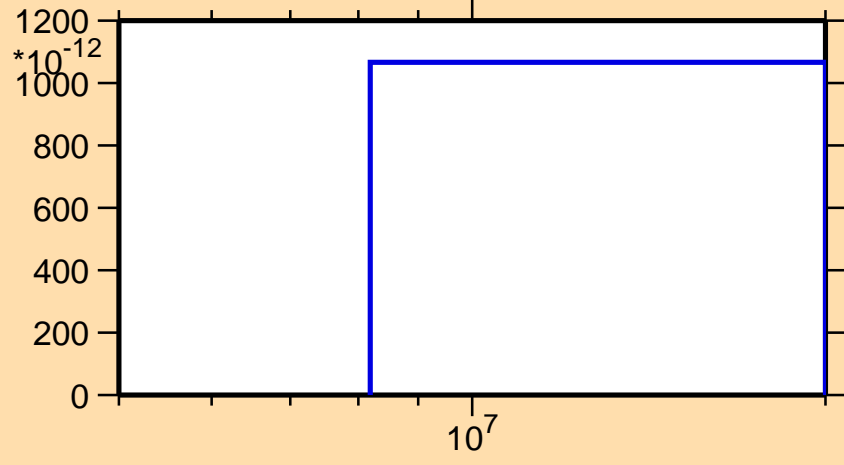
\sigma vs. E for ^{147}\text{Eu}(\text{mt117})
