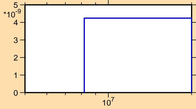
\sigma vs. E for ^{147}\text{Eu} (mt 45)
