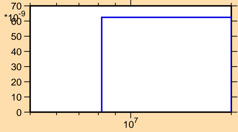
\sigma vs. E for ^{147}\text{Eu}(n,nt)
