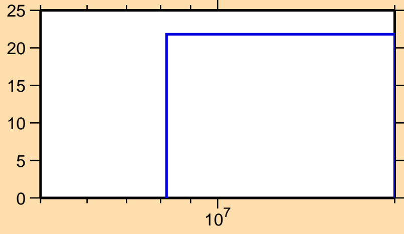
\Delta\sigma/\sigma vs. E for ^{147}\text{Eu}(n,\text{inel.})
