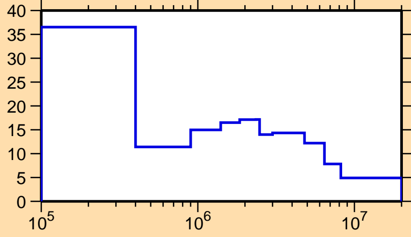
\Delta\sigma/\sigma vs. E for ^{147}\text{Eu}(n,\text{tot.})
