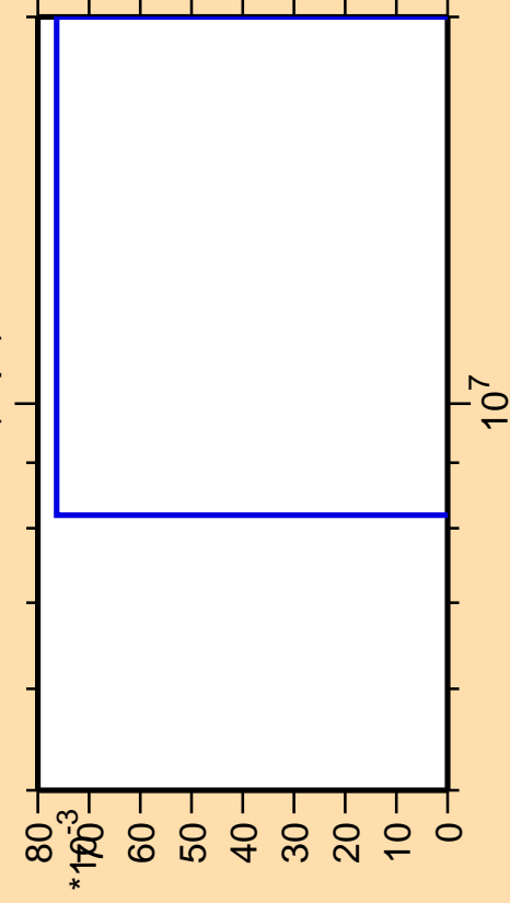
\Delta\sigma/\sigma vs. E for ^{147}\text{Eu}(n,\text{pt})
