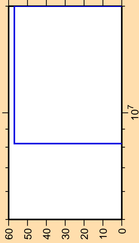
\Delta\sigma/\sigma vs. E for ^{147}\text{Eu}(n,p)
