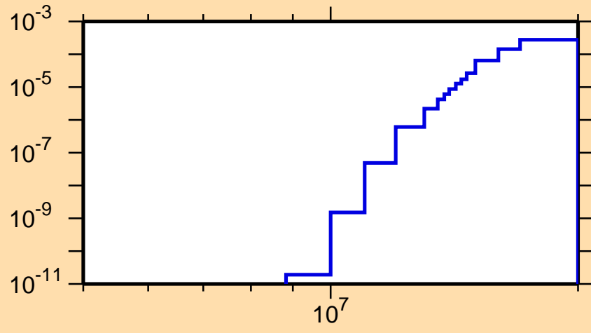
\sigma vs. E for ^{148}\text{Eu}(n,2n\alpha)
