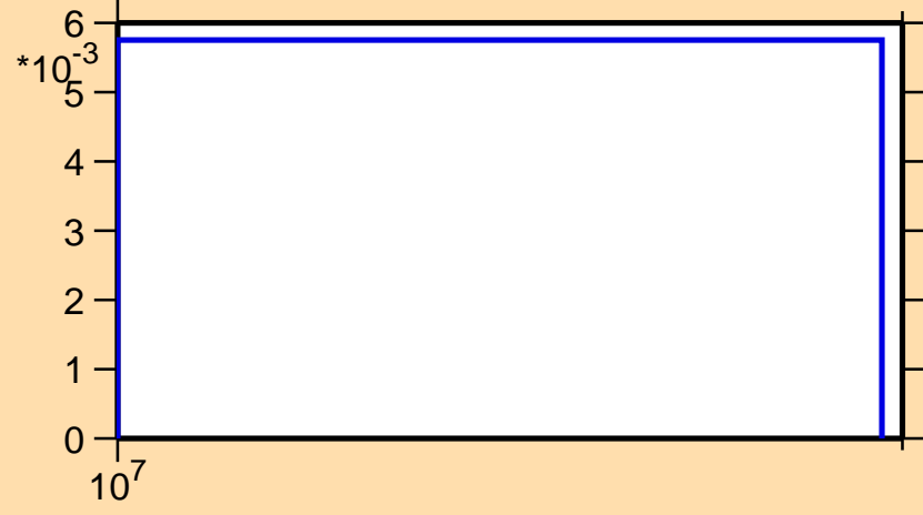
\sigma vs. E for ^{148}\text{Eu}(n,3n)
