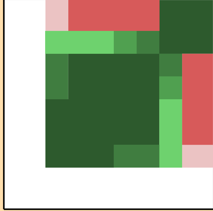
\sigma vs. E for ^{150}\text{Eu}(n,n\text{cont.})
