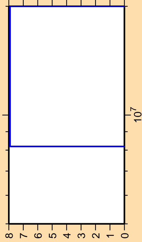
\Delta\sigma/\sigma vs. E for ^{150}\text{Eu} (mt 45)
