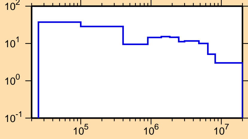
\Delta\sigma/\sigma vs. E for ^{150}\text{Eu}(n,\text{tot.})
