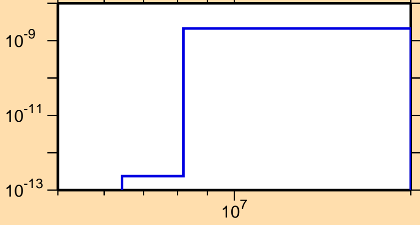
\sigma vs. E for ^{150}\text{Eu}(n,p\alpha)
