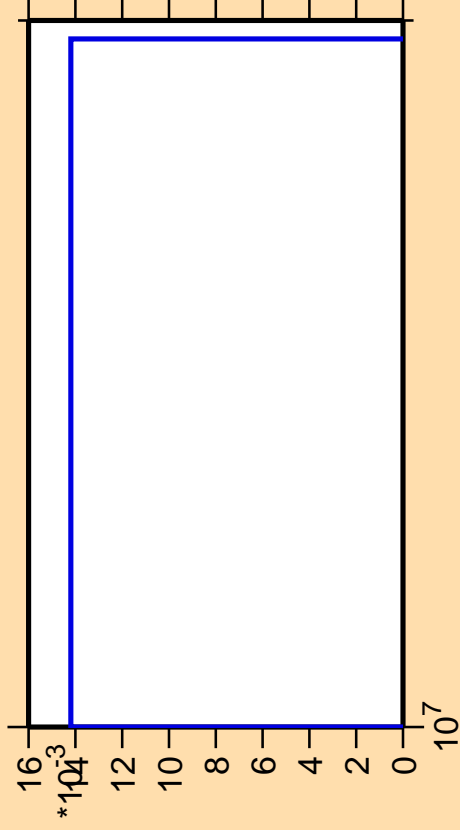
\Delta\sigma/\sigma vs. E for ^{150}\text{Eu} (mt 11)
