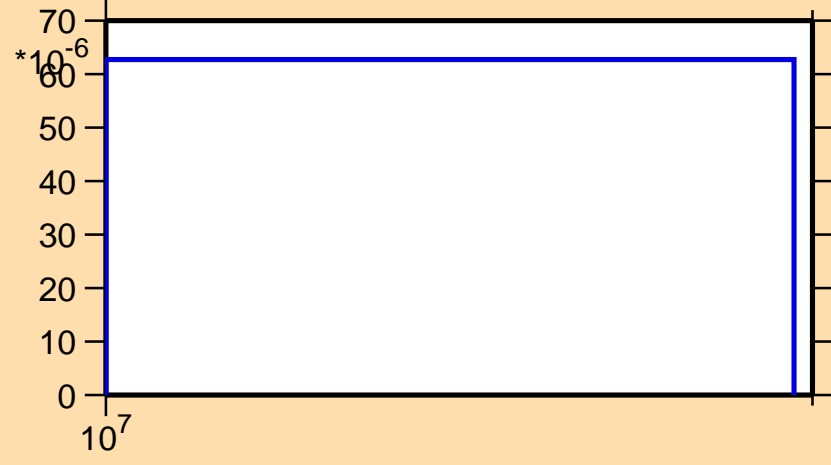
\sigma vs. E for ^{150}\text{Eu}(n,2np)
