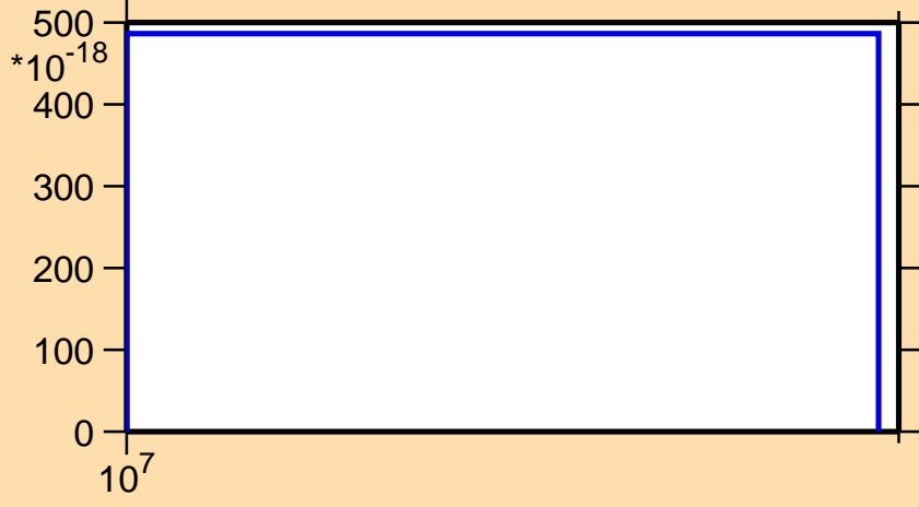
\sigma vs. E for ^{150}\text{Eu}(n,\text{pt})
