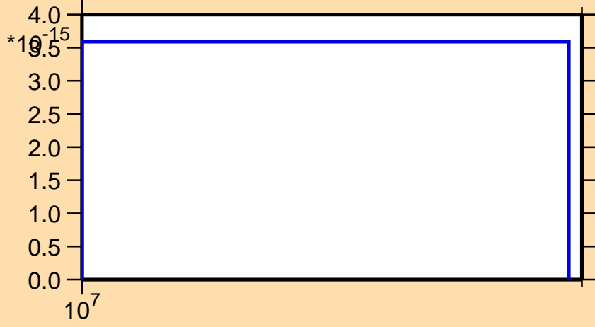
\sigma vs. E for ^{150}\text{Eu} (mt 11)
