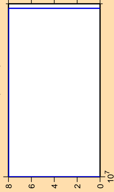
\Delta\sigma/\sigma vs. E for ^{150}\text{Eu}(n,3n\alpha)
