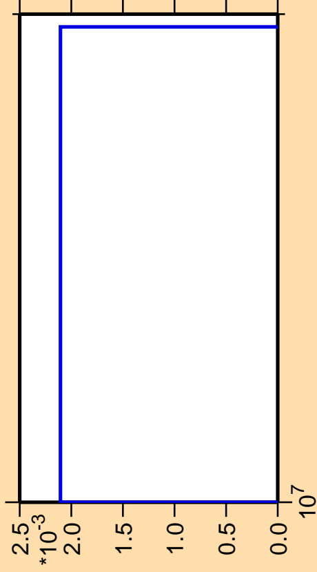
\Delta\sigma/\sigma vs. E for ^{150}\text{Eu}(n,\text{pt})
