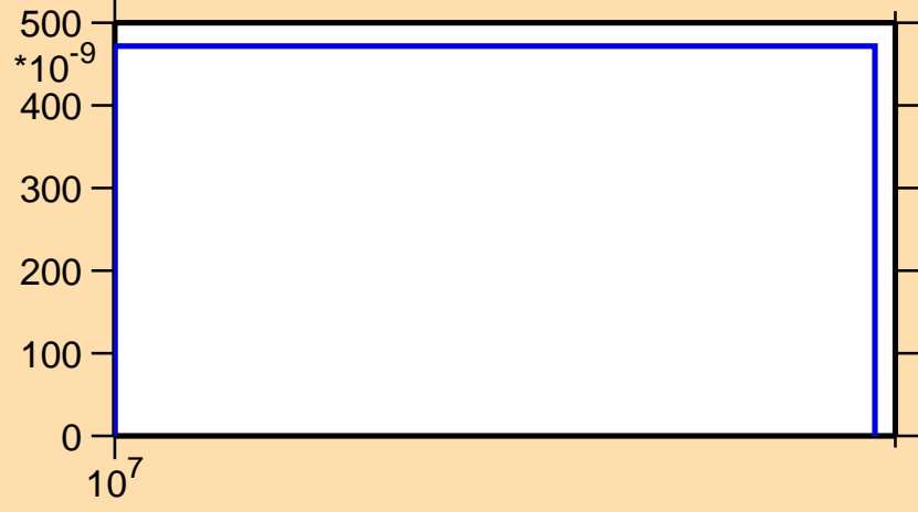
\sigma vs. E for ^{150}\text{Eu}(n,nt)
