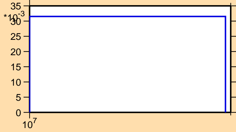
\sigma vs. E for ^{150}\text{Eu}(n,3n)
