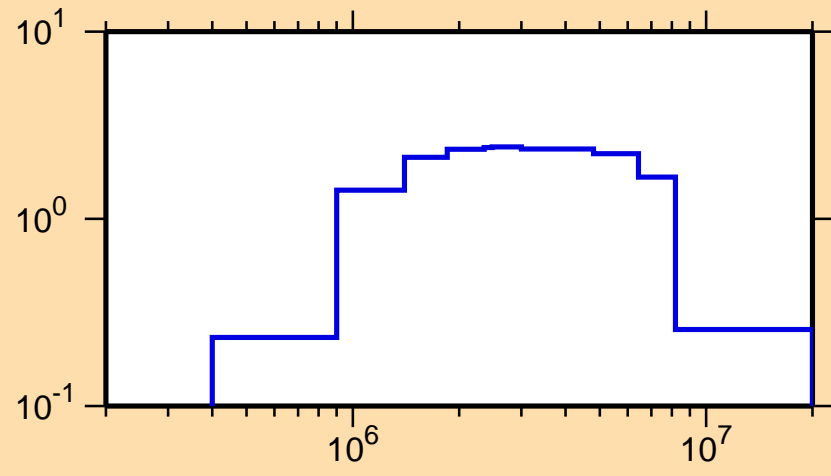
\sigma vs. E for ^{150}\text{Eu}(n,n\text{cont.})
