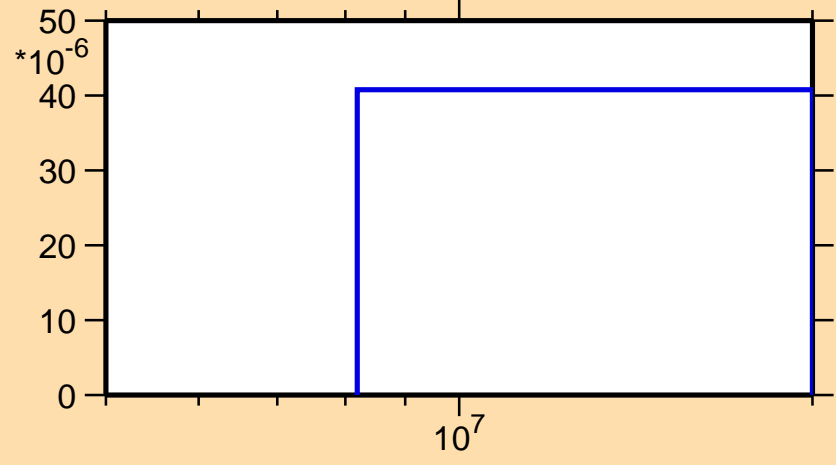
\sigma vs. E for ^{150}\text{Eu}(n,2n\alpha)
