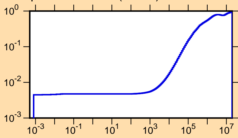
\mu vs. E for ^{151}\text{Eu}(\text{mt251})
