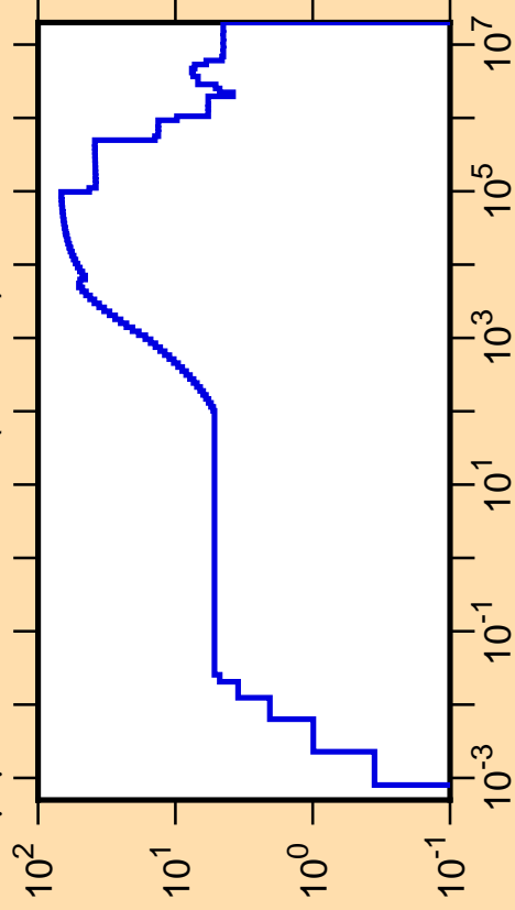
\Delta\mu/\mu vs. E for ^{151}\text{Eu}(\text{mt251})
