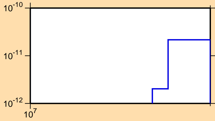
\sigma vs. E for ^{151}\text{Eu} (mt 45)
