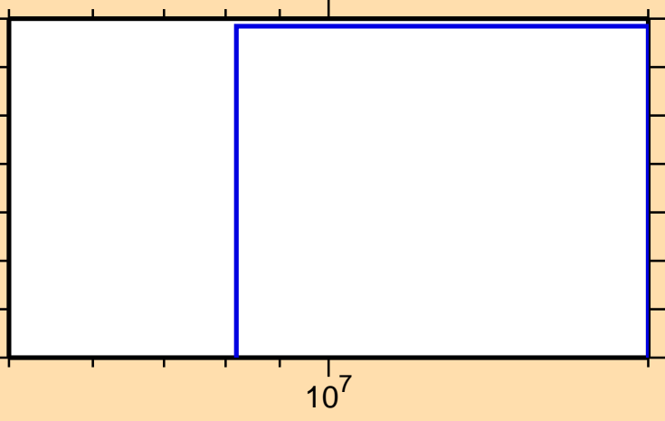
\sigma vs. E for ^{151}\text{Eu}(n,2n\alpha)
