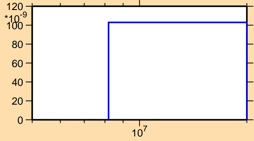
\sigma vs. E for ^{151}\text{Eu}(n,nt)
