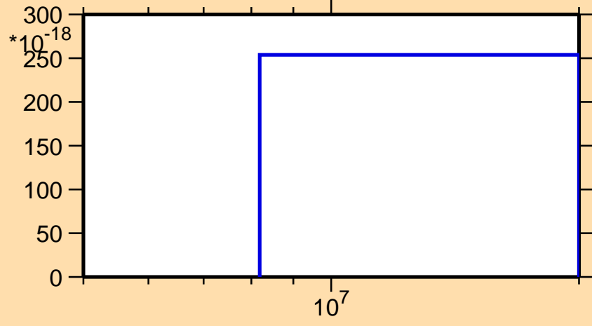
\sigma vs. E for ^{151}\text{Eu} (mt 11)
