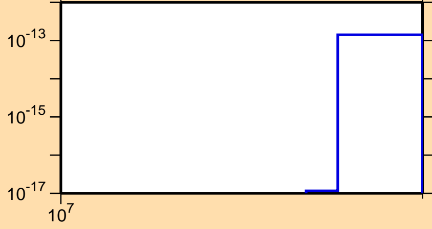
\sigma vs. E for ^{152}\text{Eu} (mt 34)
