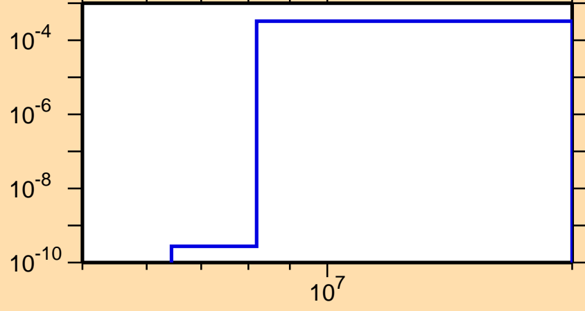
\sigma vs. E for ^{152}\text{Eu}(n,t)
