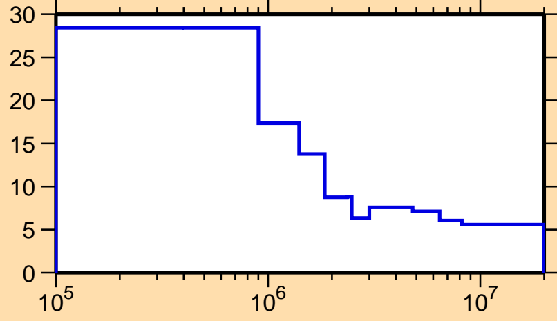
\Delta\sigma/\sigma vs. E for ^{152}\text{Eu}(n,n\text{onel.})
