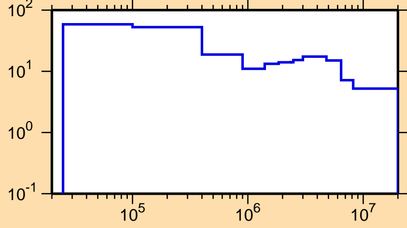
\Delta\sigma/\sigma vs. E for ^{152}\text{Eu}(n,\text{el.})
